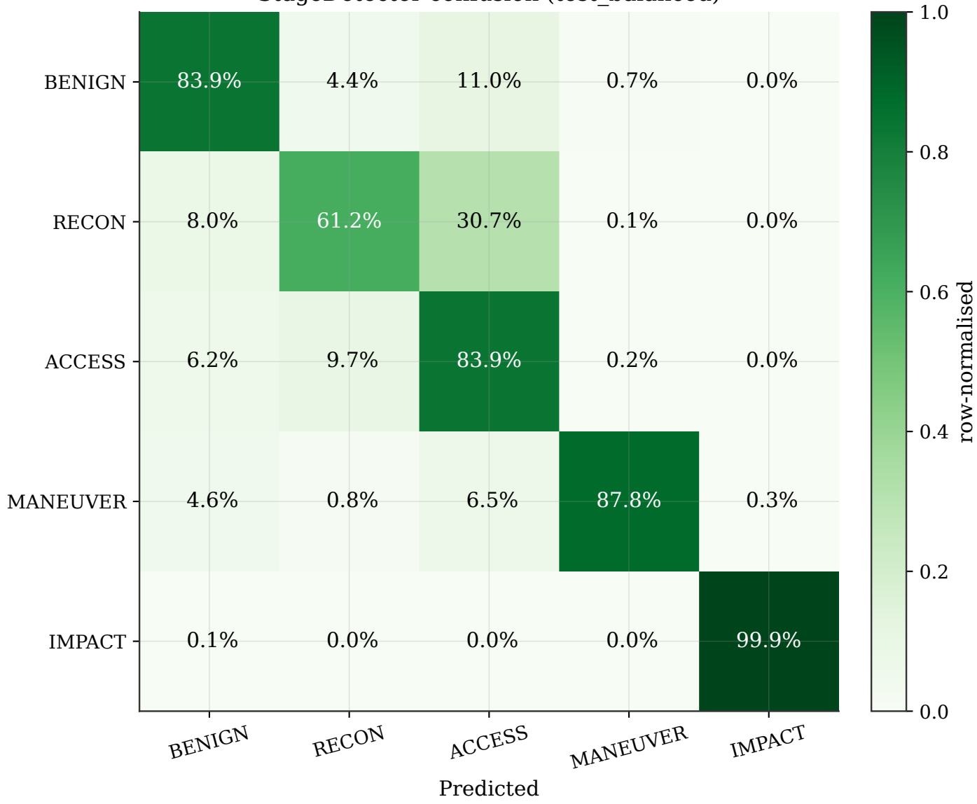
StageDetector confusion (test_balanced)
