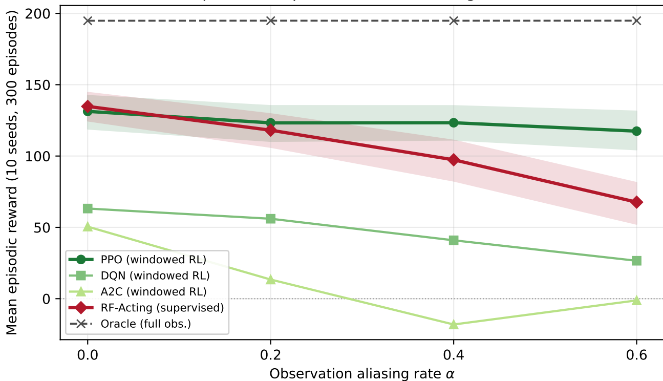
Windowed RL holds under partial observability; the per-flow supervised classifier degrades
