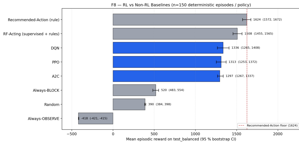
Figura 4.6 – Mean episodic reward with 95 % bootstrap confidence intervals on the held-out test_balanced split. The oracle Recommended-Action rule (marker (o) ) reads the true attack stage from the simulator and is a measurement instrument, not a competing baseline. Among deployable policies the ranking is RF-Acting > trained DRL > Always-BLOCK > Random > Always-OBSERVE.
