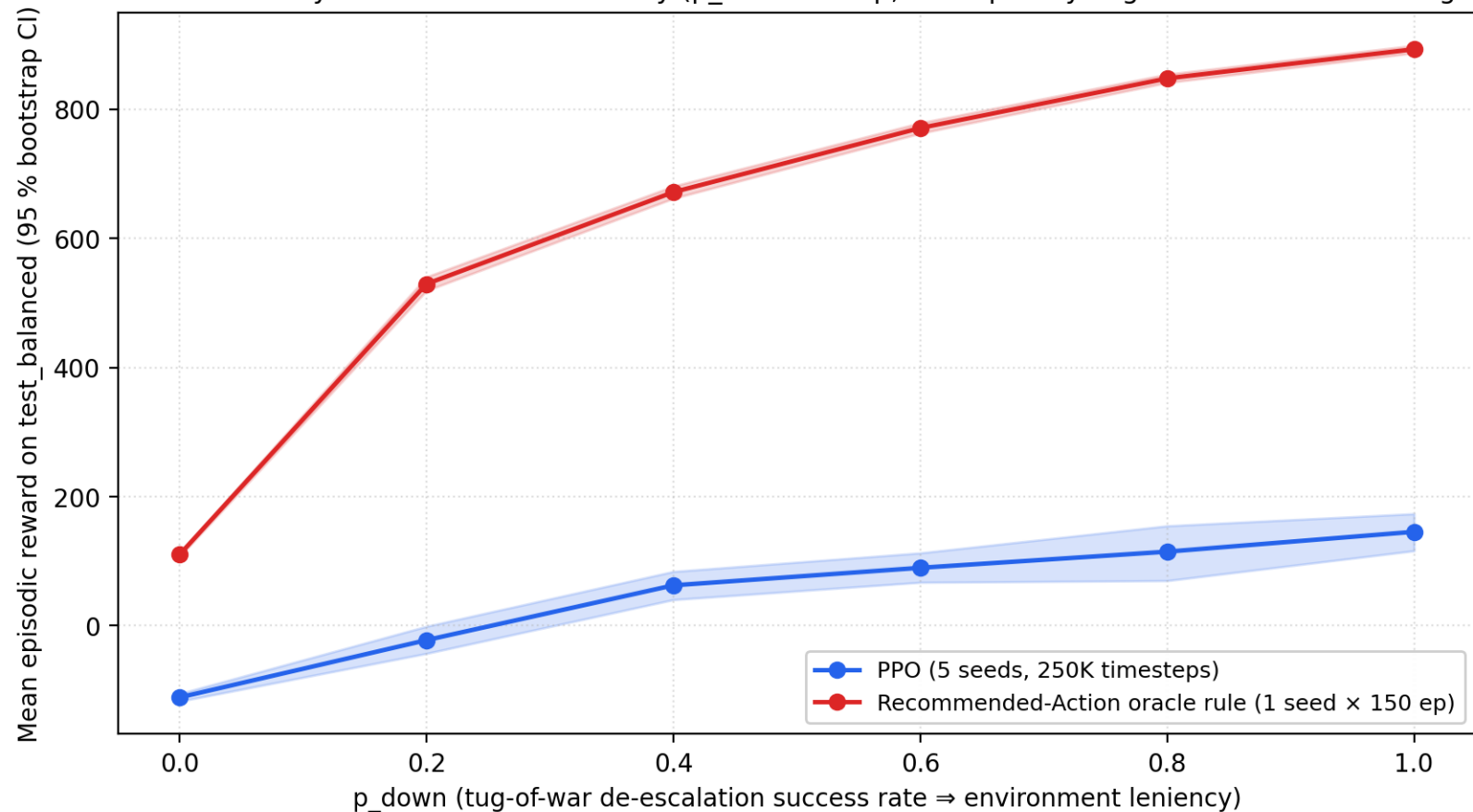
F10 — Sensitivity to environment difficulty (p_down sweep; conceptually aligned with IoTWarden Fig. 6)
