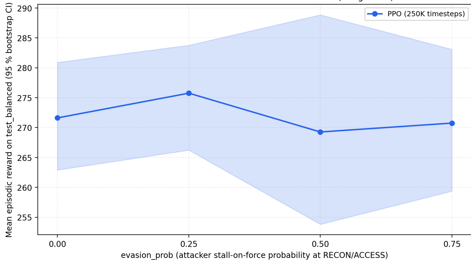
F17 — Defender robustness to an evasive attacker (budget=40)
