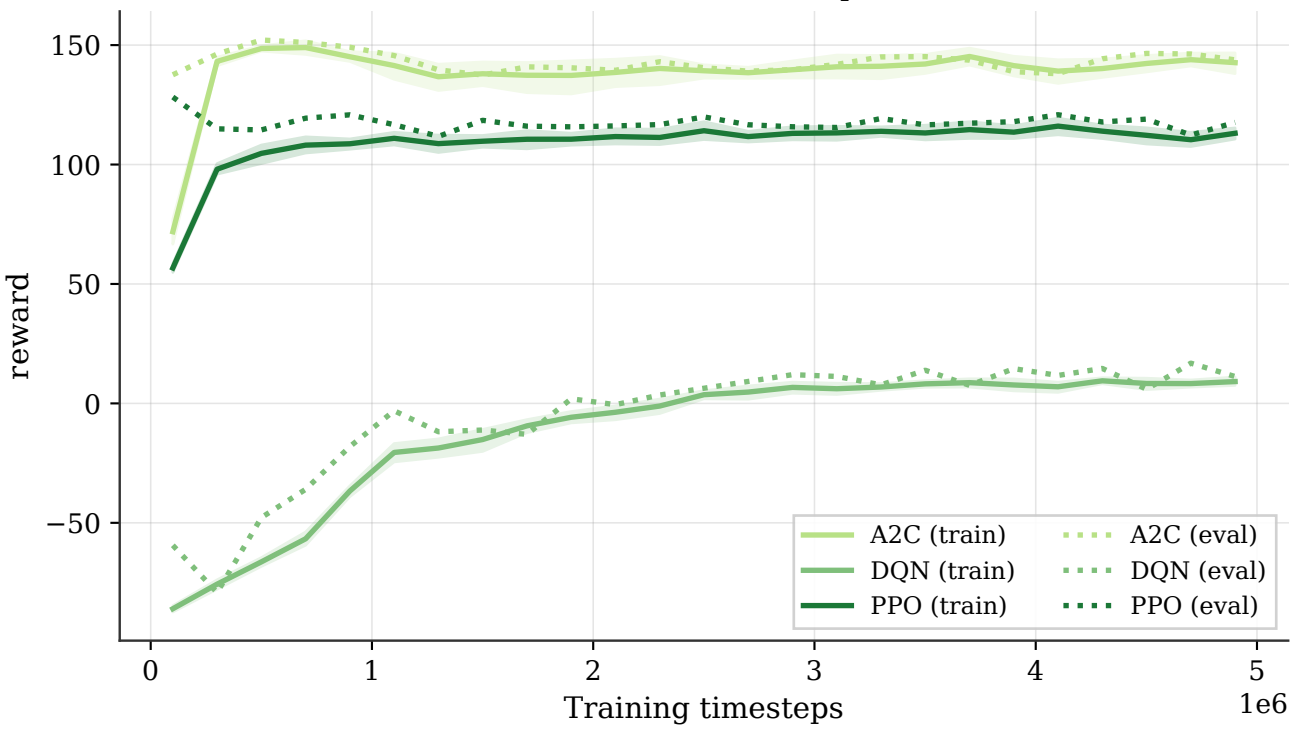
Mean episodic reward over training (A2C/DQN/PPO, 10 seeds per algorithm; 25 time bins; bands = 95 % bootstrap CI across seeds)
