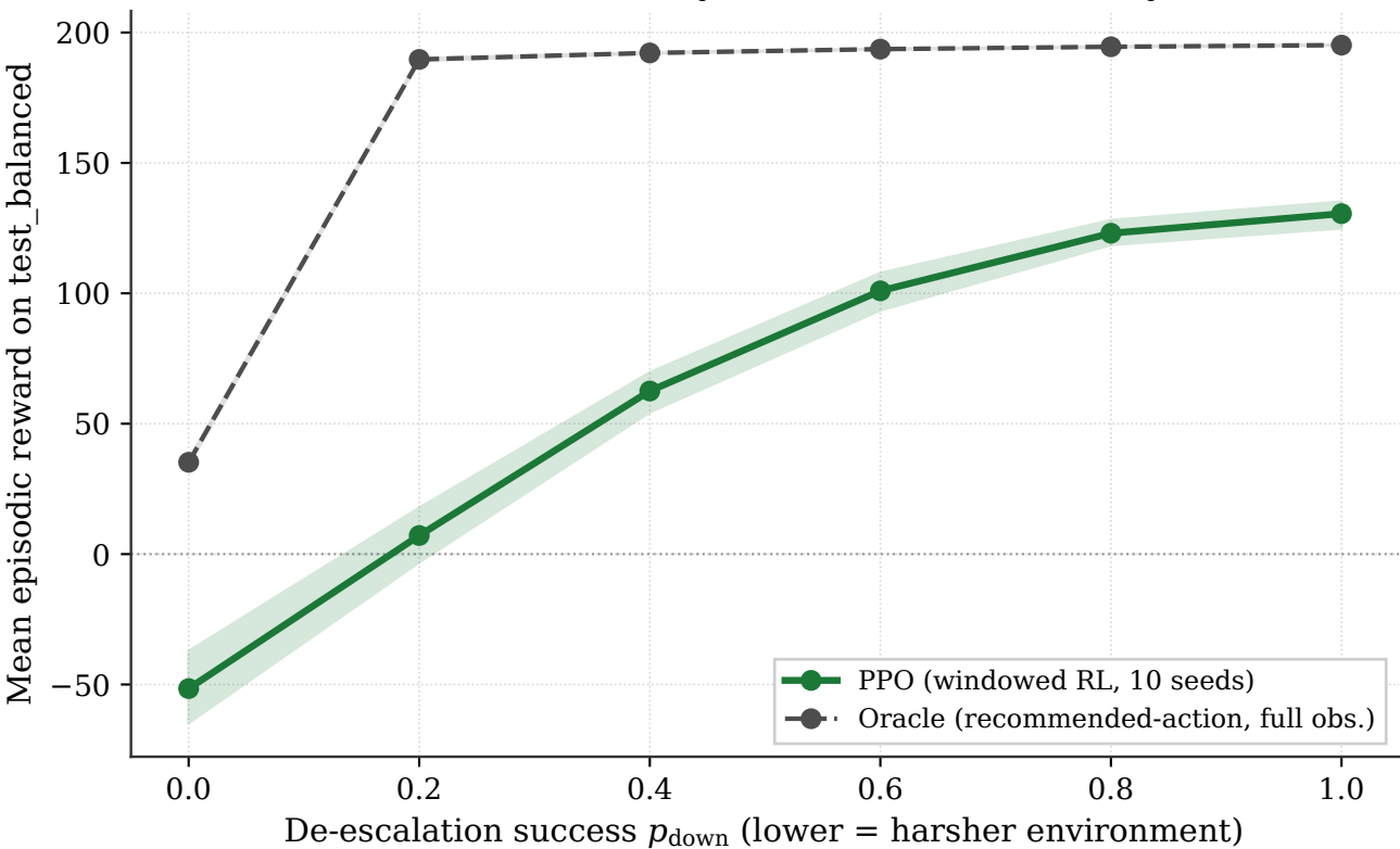
Defender sensitivity to environment difficulty
