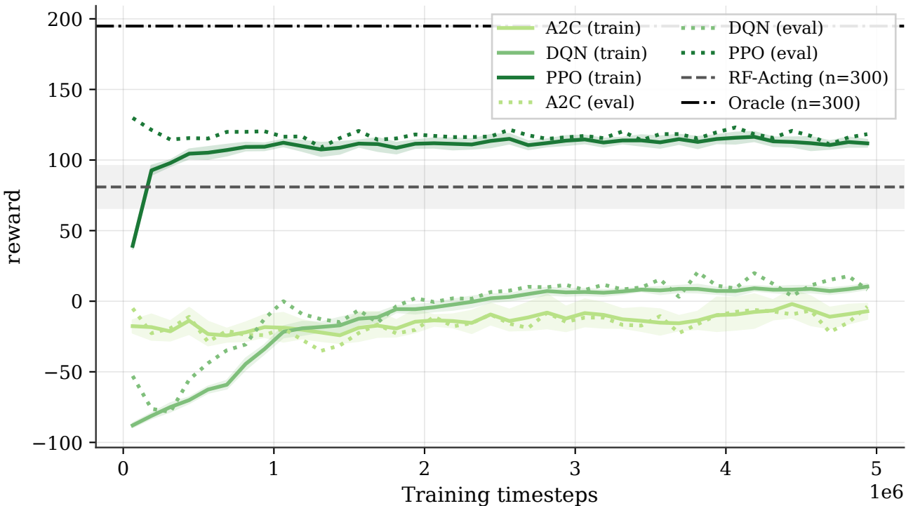
Mean episodic reward over training (A2C/DQN/PPO, 10 seeds per algorithm; 40 time bins; bands = 95 % bootstrap CI across seeds)
