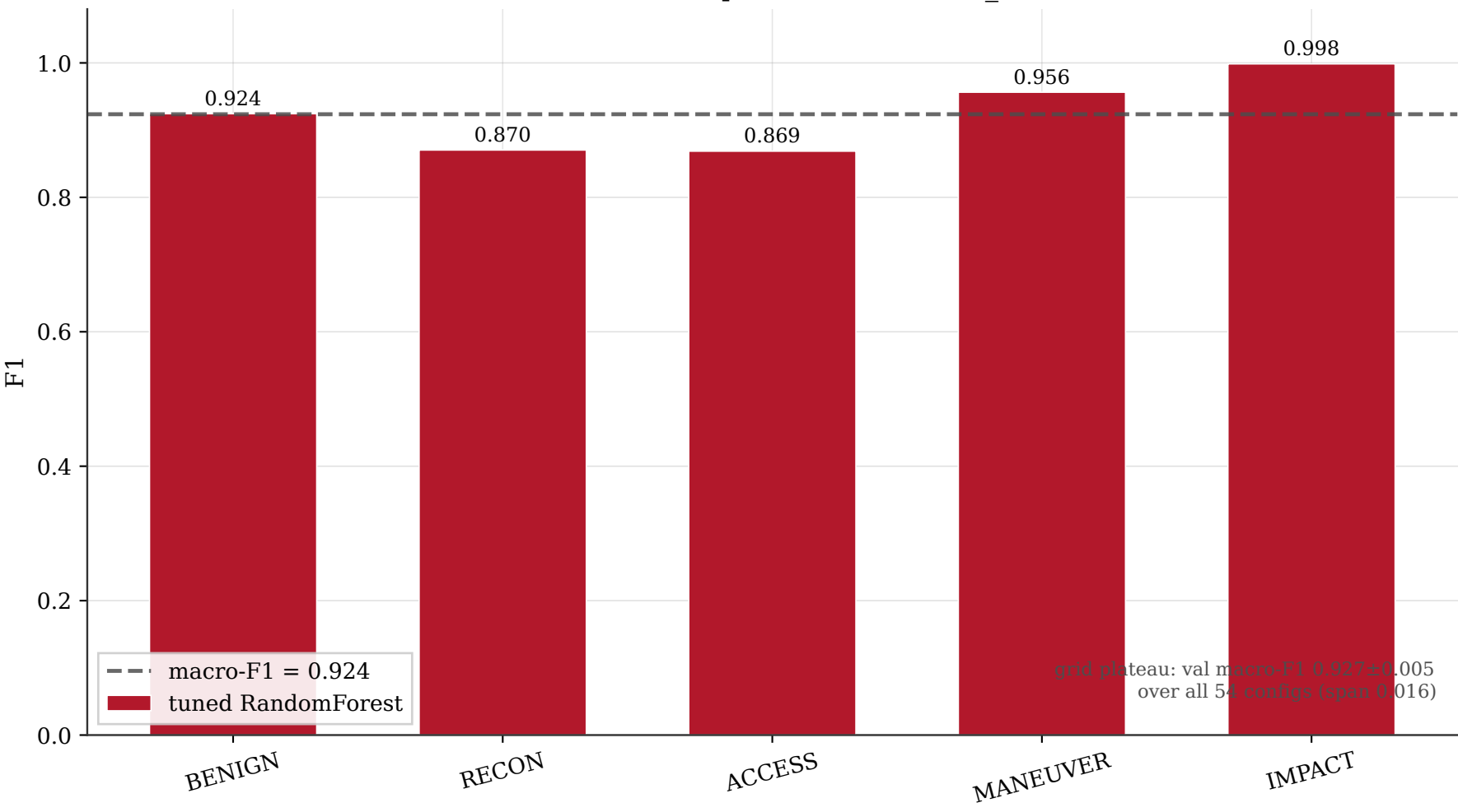
Tuned RandomForest per-class F1 on test_balanced
