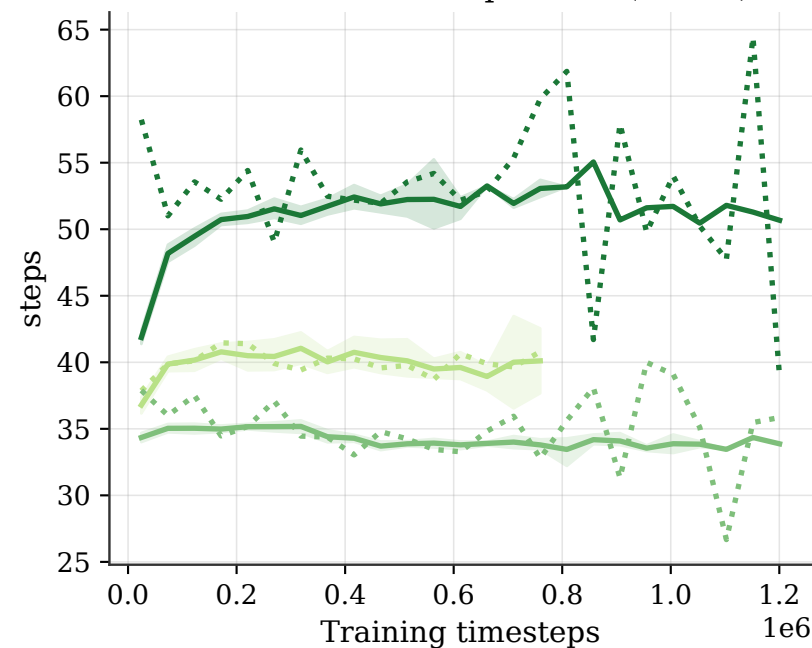
Mean Time-To-Compromise (MTTC)
