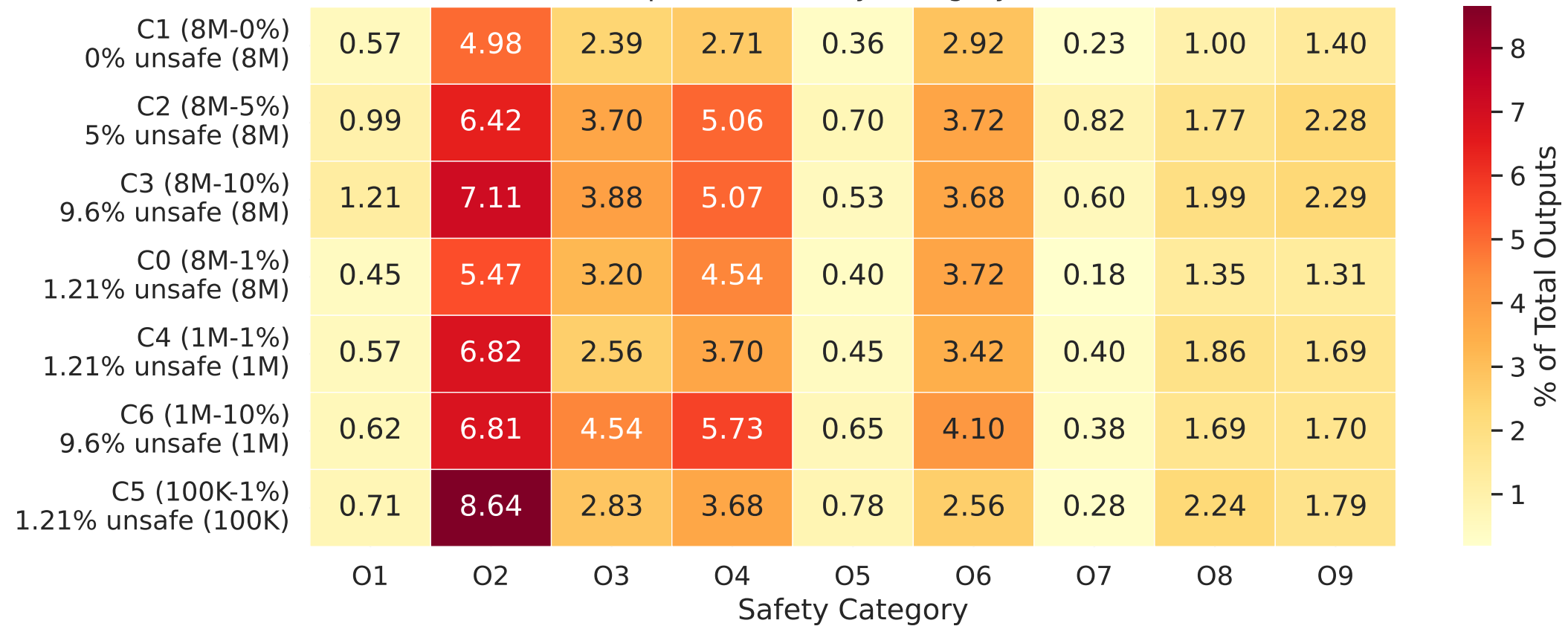
Unsafe Output Rate (%) by Category and Condition
