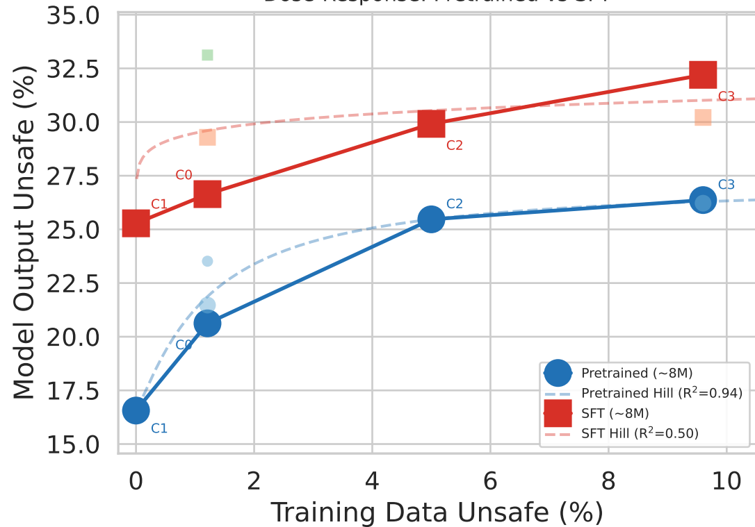
Dose-Response: Pretrained vs SFT
