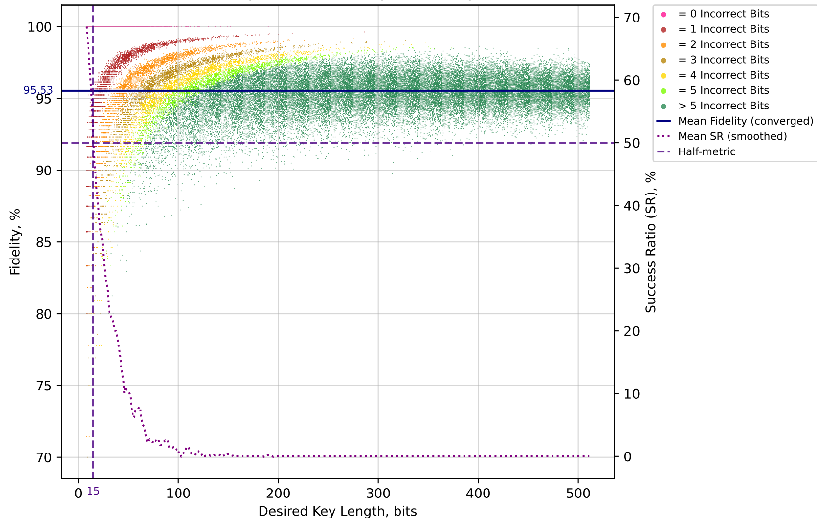
B92 Fidelity Simulation - High Error Regime
