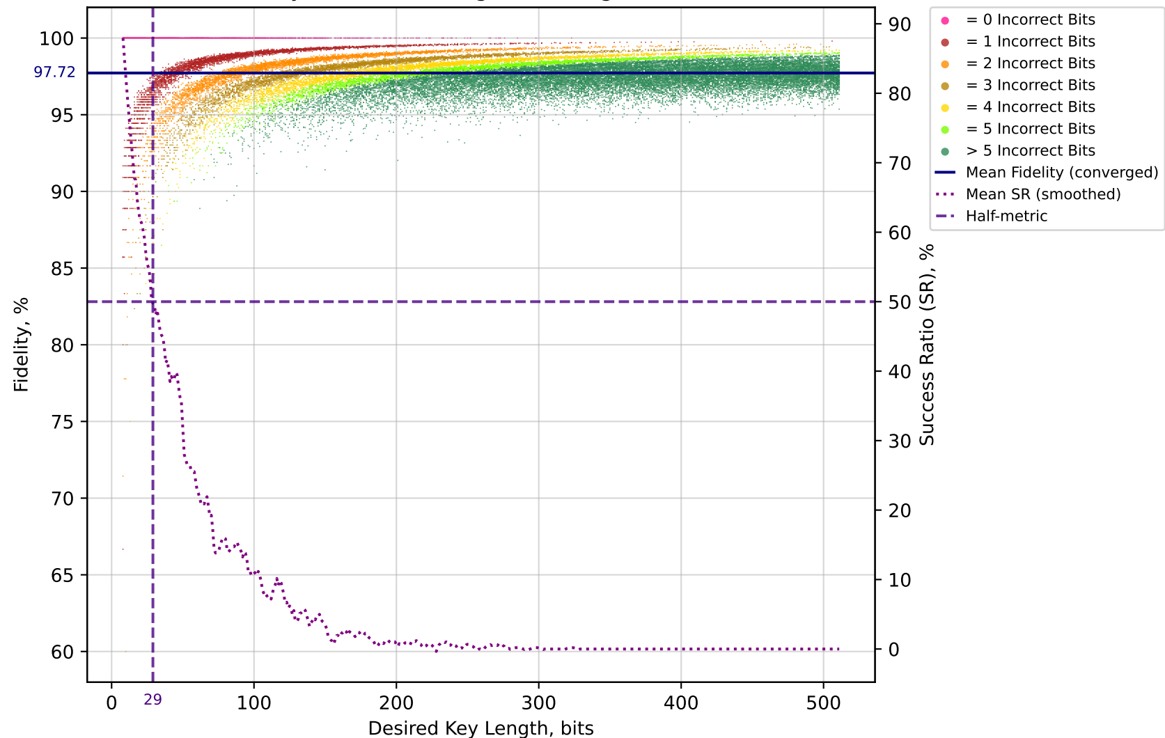
B92 Fidelity Simulation - High Error Regime Normalised
