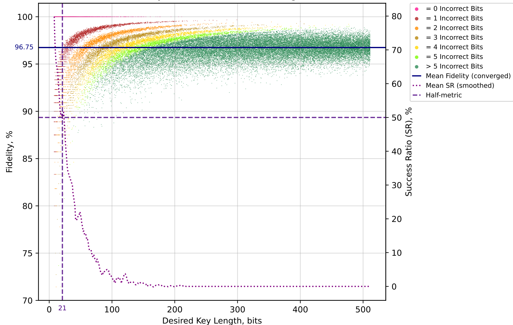
B92 Fidelity Simulation - Low Error Regime
