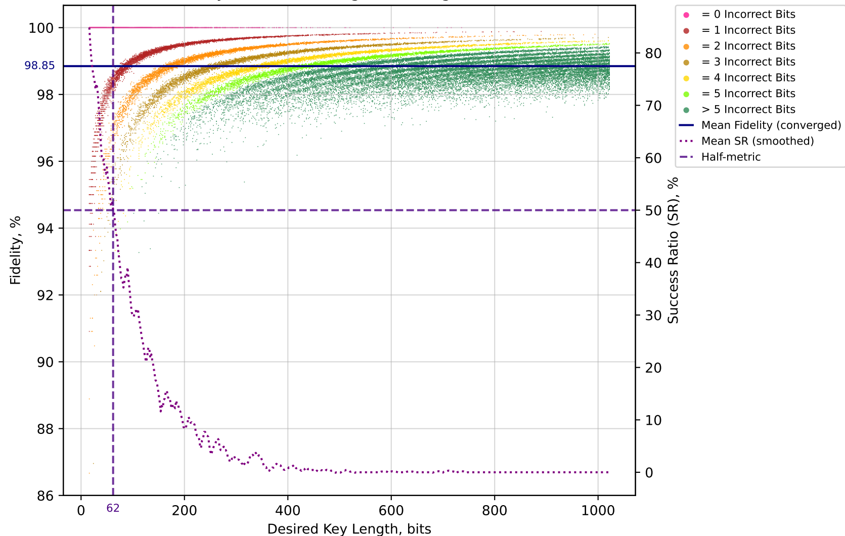
BB84 Fidelity Simulation - High Error Regime Normalised
