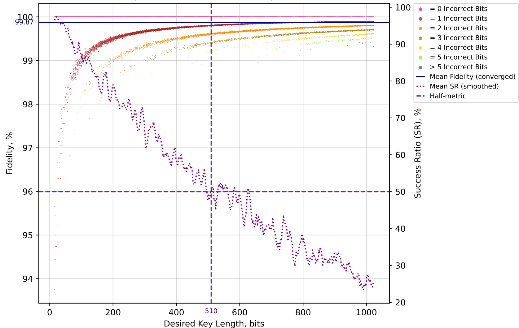
BB84 Fidelity Simulation - Low Error Regime Normalised
