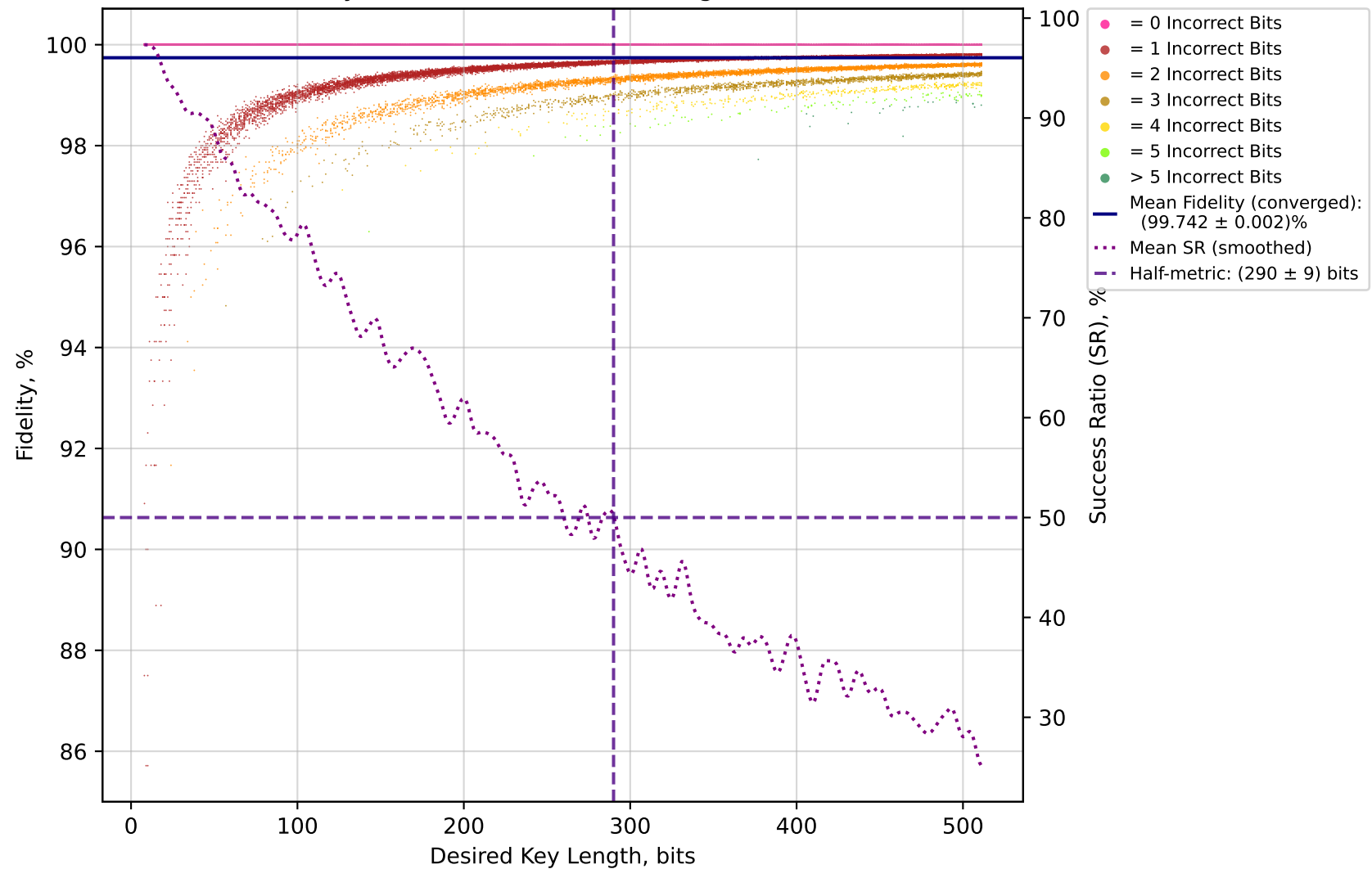
B92 Fidelity Simulation - Low Error Regime Normalised
