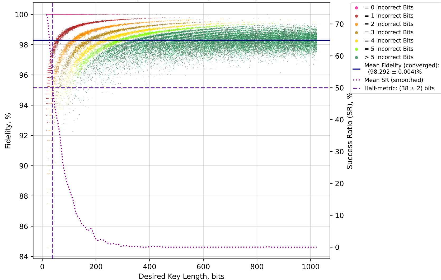
BB84 Fidelity Simulation - High Error Regime
