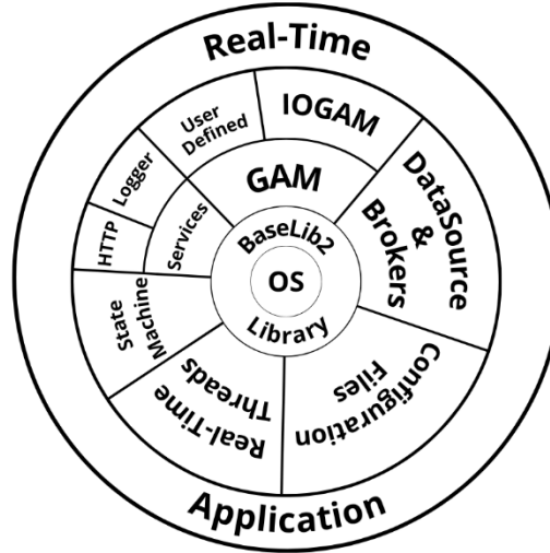
Figure 10: Core MARTe2 components for real-time applications
