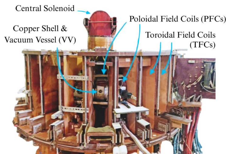
Figure 5: Frontal view of ISTTOK, highlighting its main components (adapted from [40, p. 2])
