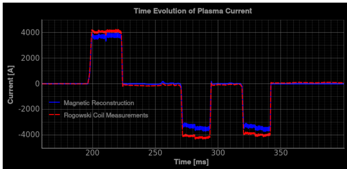
Figure 22: Comparison of plasma current obtained from magnetic reconstruction and Rogowski coil measurements for shot 53071
