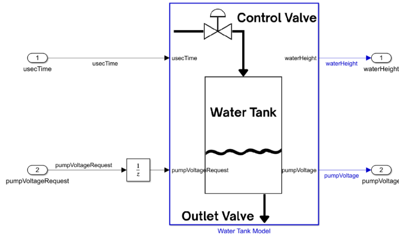
Figure 18: Simulink water tank model for MARTe2 integration
