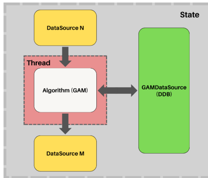
Figure 13: Overview of the structure of the simplest functional MARTe real-time application
