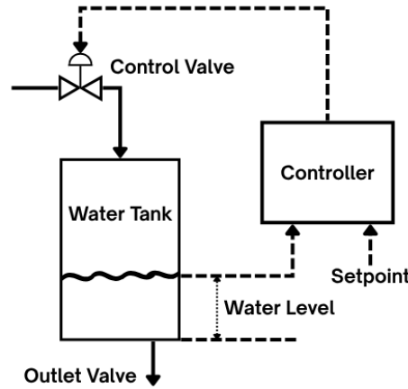
Figure 15: Water tank model used for feedback control analysis
