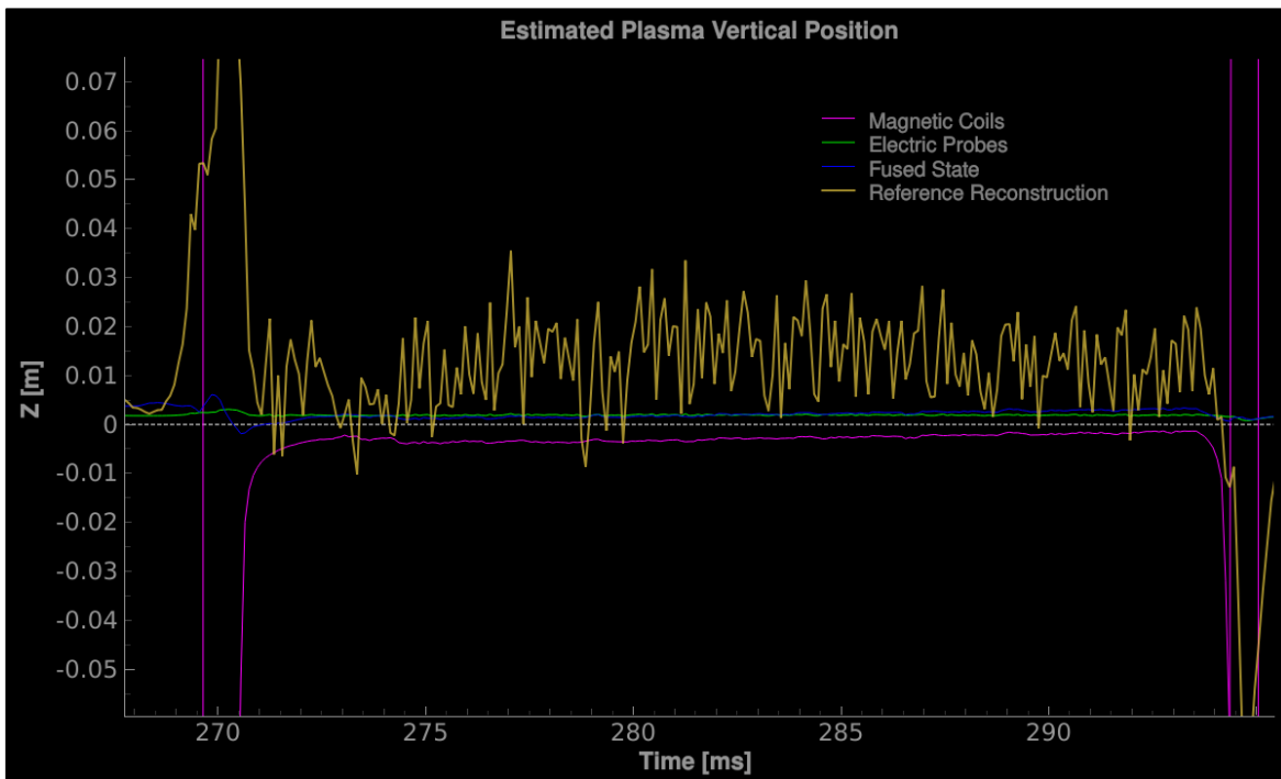
Figure 27: Plasma vertical position for shot 53071 estimated by magnetic coils, electric probes, fused state, and reference reconstructions
