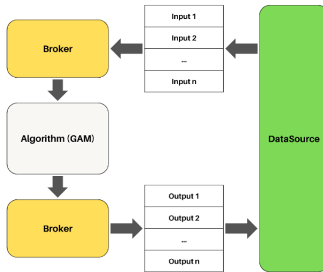
Figure 12: Overview of the communication logic managed by DataSources and supervised by Brokers
