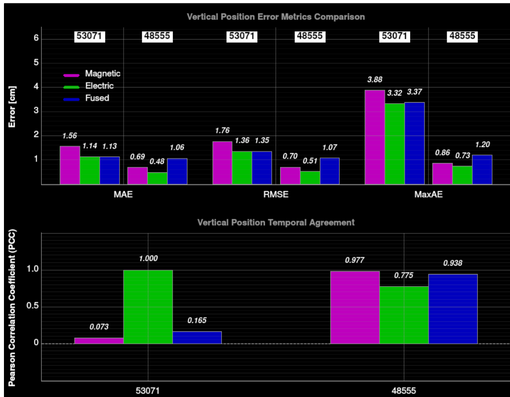
Figure 31: Plasma vertical position estimation metrics for magnetic coils, electric probes, and fused state, using the reference reconstruction as benchmark
