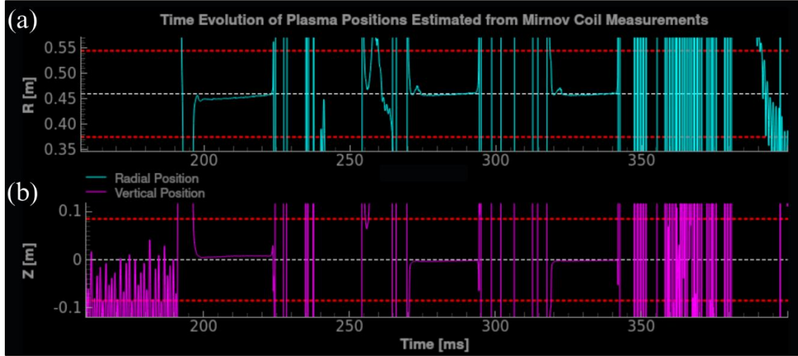
Figure 23: (a) Radial and (b) vertical plasma positions reconstructed from magnetic measurements for shot 53071
