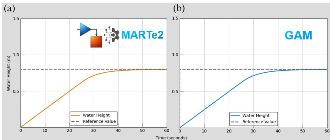
Figure 19: Water tank feedback control system response (a) using the Simulink water model integrated into MARTe2 with the ‘SimulinkWrapperGAM’ and (b) using the ‘WaterTankGAM’
