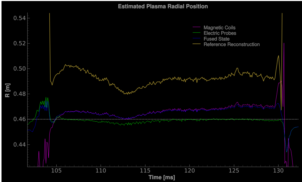
Figure 28: Plasma radial position for shot 48555 estimated by magnetic coils, electric probes, fused state, and reference reconstructions
