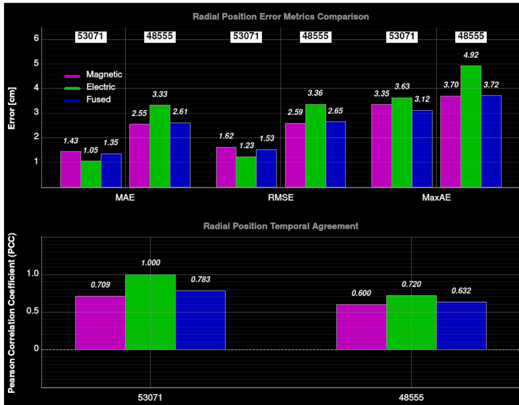
Figure 30: Plasma radial position estimation metrics for magnetic coils, electric probes, and fused state, using the reference reconstruction as benchmark
