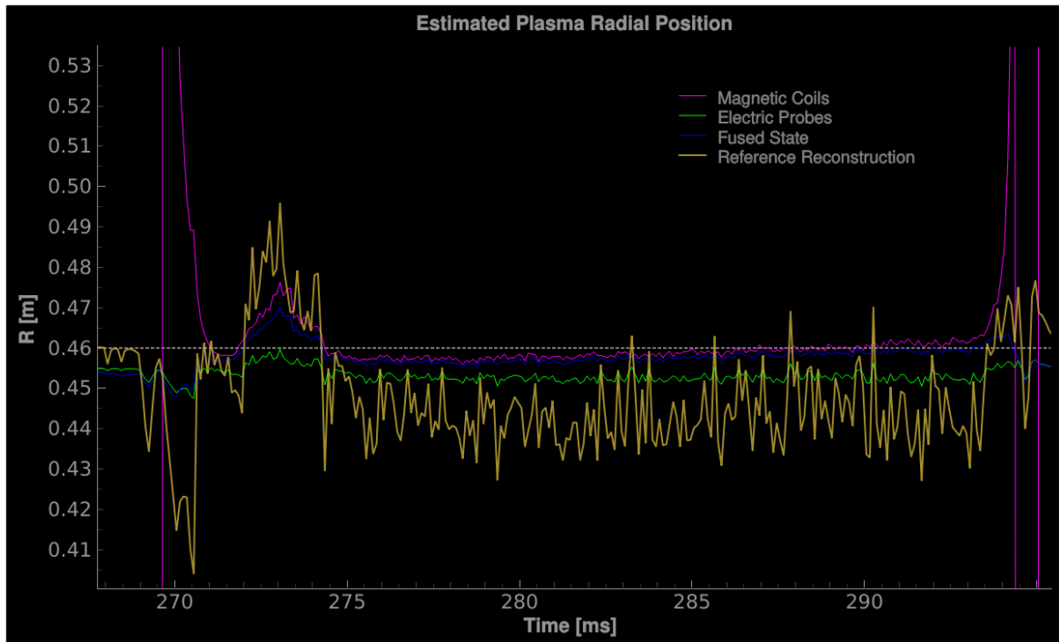
Figure 26: Plasma radial position for shot 53071 estimated by magnetic coils, electric probes, fused state, and reference reconstructions
