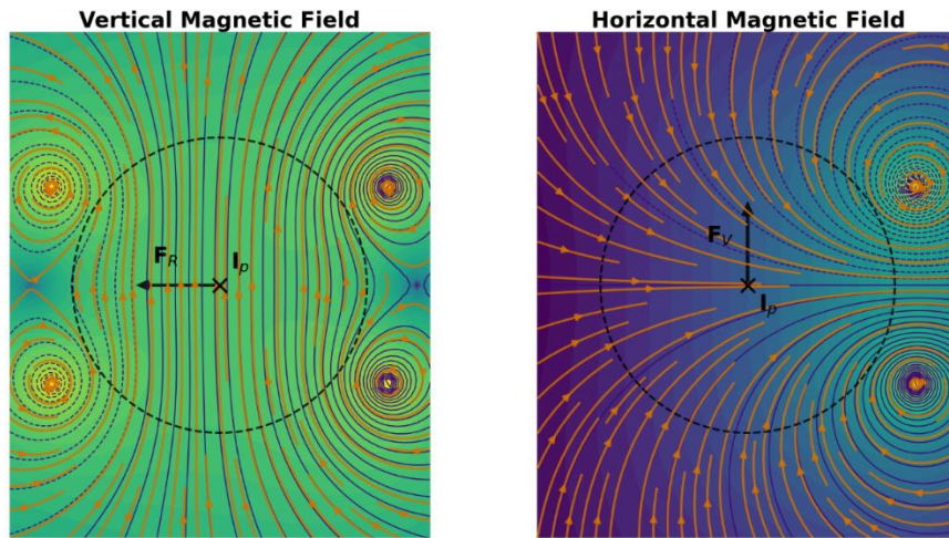
Figure 4: Illustration of poloidal magnetic fields and the resulting forces under idealized conditions
