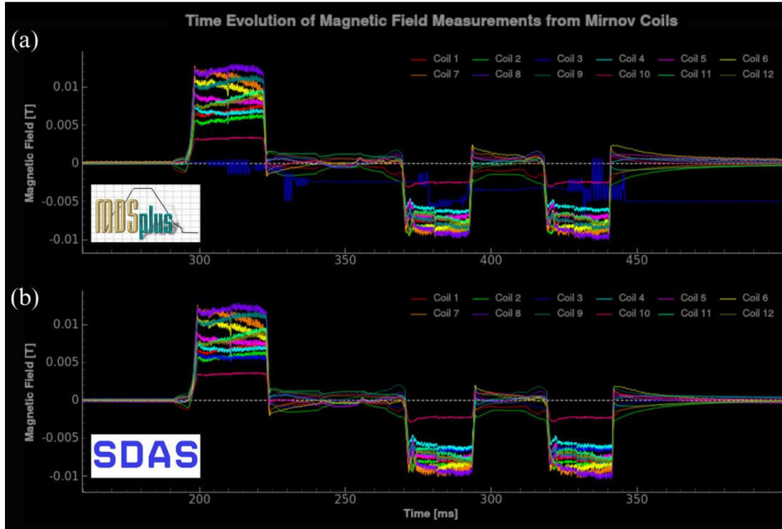
Figure 21: Time evolution of magnetic field measurements from 12 Mirnov coils for shot 53071 (a) using MDSplus (new ATCA board); (b) using the ISTTOK Shared Data Access System (old ATCA board)
