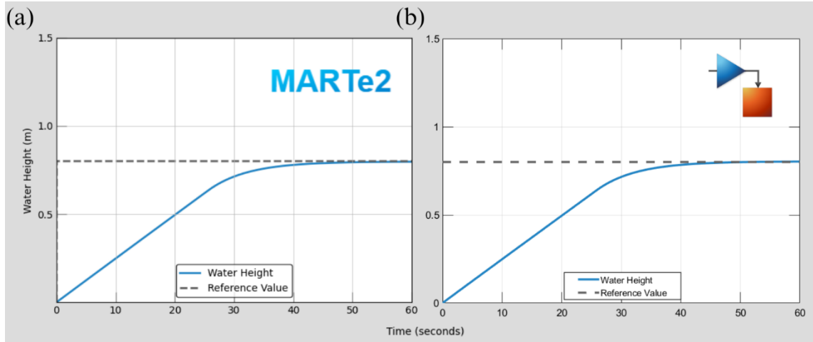
Figure 17: (a) Water tank feedback control system response in MARTe2; (b) Water tank feedback control system response in Simulink
