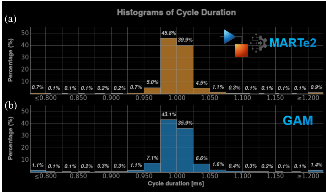
Figure 20: (a) Cycle duration histogram using the Simulink water model integrated into MARTe2 with the 'SimulinkWrapperGAM'; (b) Cycle duration histogram using the 'WaterTankGAM'
