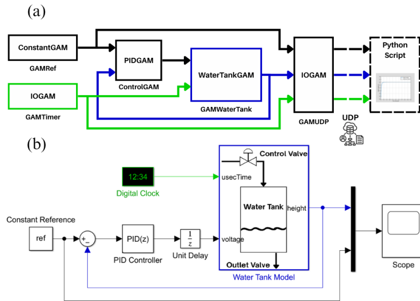
Figure 16: (a) Block-based representation of MARTe configuration used for simulation of the water tank feedback controlled model; (b) Simulink water tank model used for feedback control analysis
