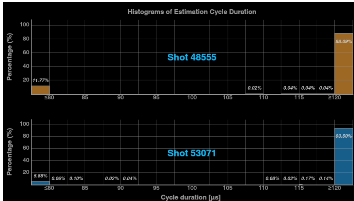
Figure 32: Estimation-cycle duration histograms for shots 48555 and 53071 evaluated around the nominal 100 \mu\text{s} real-time cycle duration
