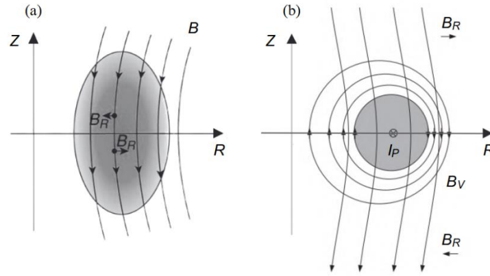
Figure 3: Vertical instability in different plasma configurations. (a) Source of vertical instability in a VE plasma (adapted from [9, p. 4]); (b) Source of vertical instability in a circular plasma (adapted from [11, p. 9])
