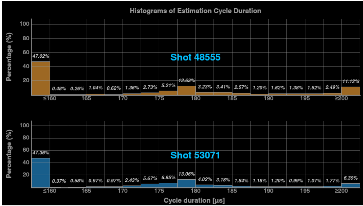
Figure 33: Estimation-cycle duration histograms for shots 48555 and 53071 evaluated in the 160-200 \mu\text{s} interval
