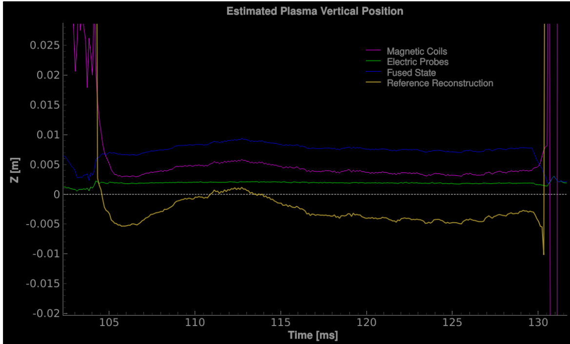
Figure 29: Plasma vertical position for shot 48555 estimated by magnetic coils, electric probes, fused state, and reference reconstructions
