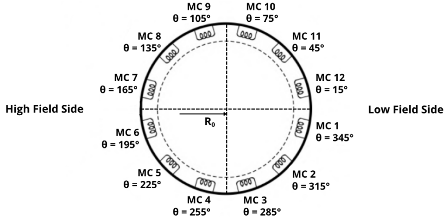
Figure 8: Illustration of ISTTOK's poloidal cross-section containing the set of Mirnov coils (adapted from [40, p. 3])
