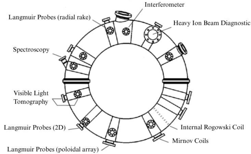
Figure 7: Overview of the main ISTTOK's diagnostics
