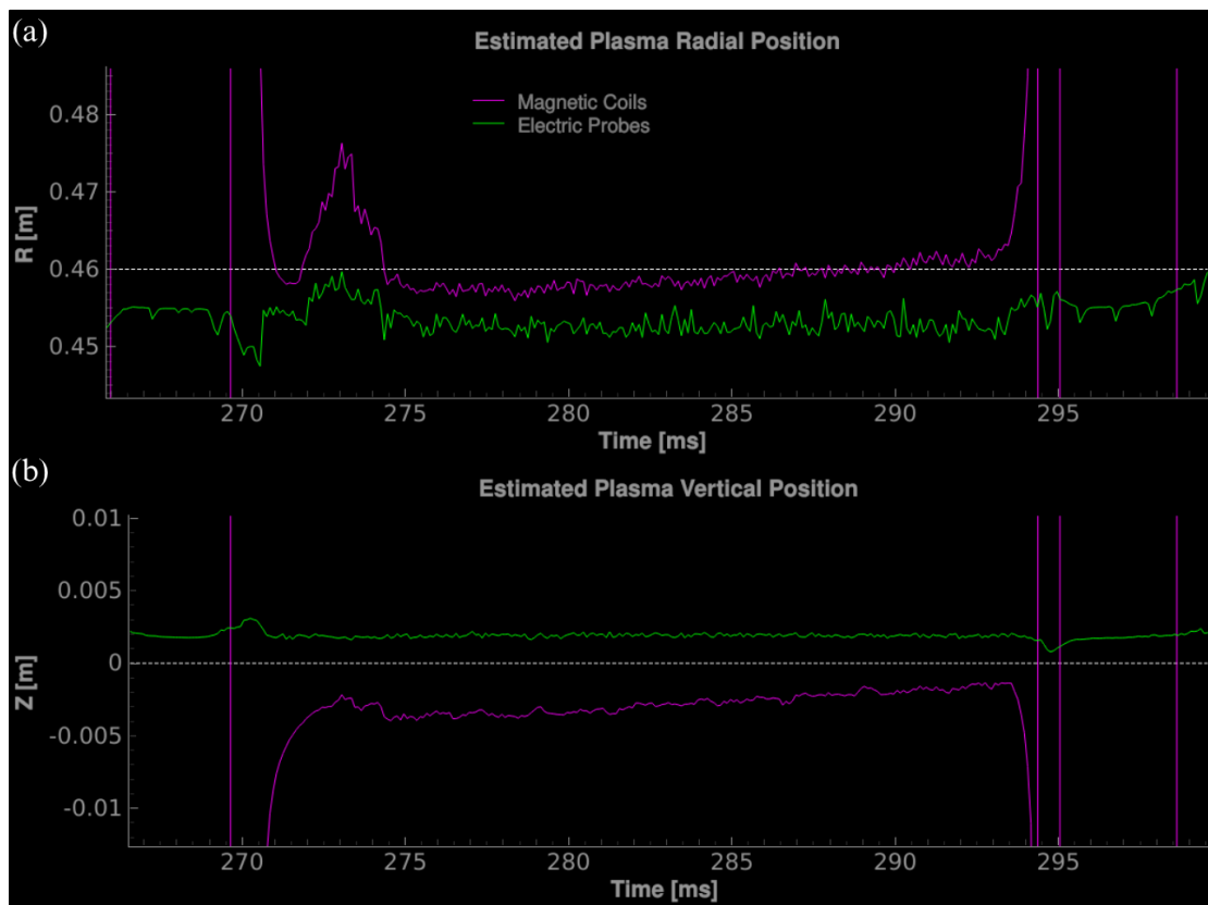
Figure 24: Comparison between (a) radial and (b) vertical plasma positions reconstructed from magnetic and electric measurements for shot 53071
