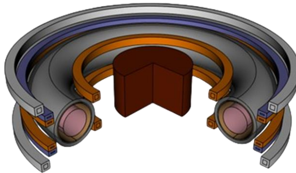
Figure 6: Simplistic illustration of ISTTOK tokamak
