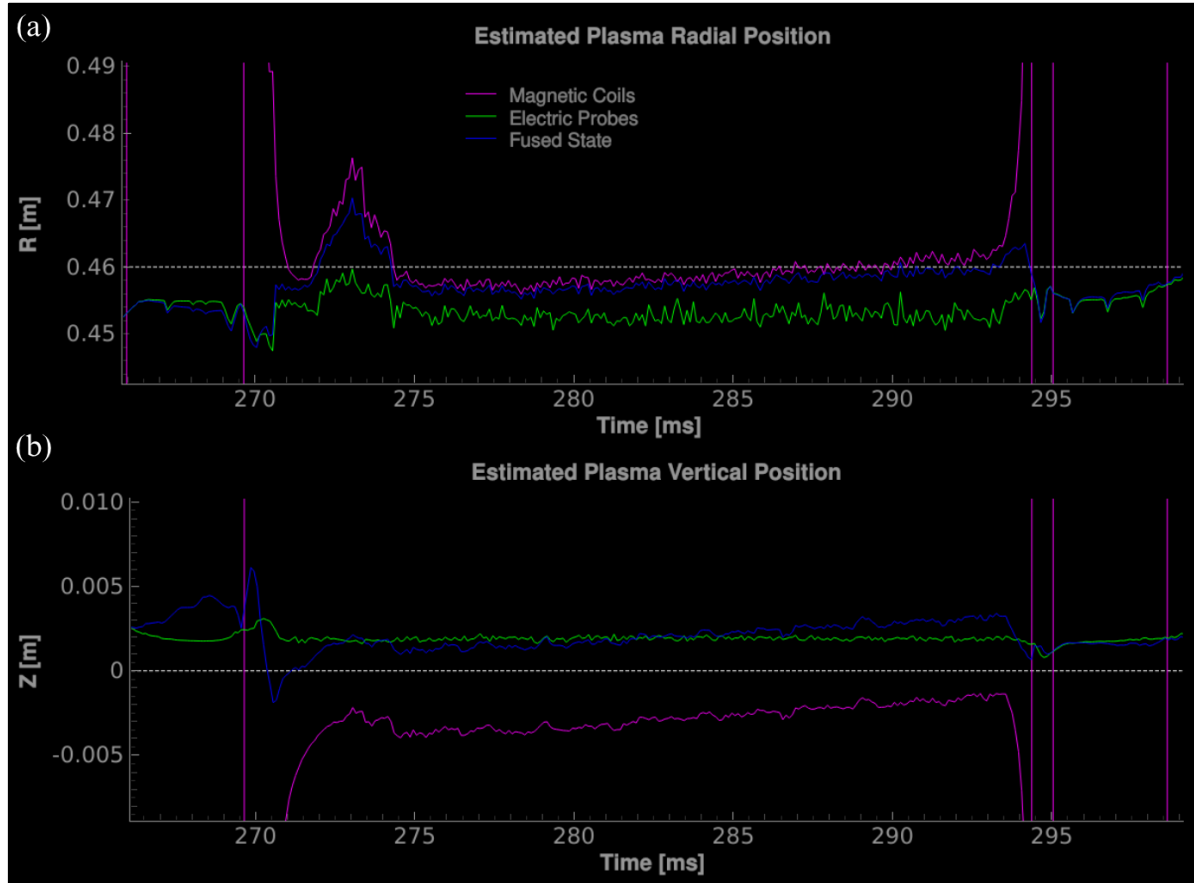
Figure 25: Estimated plasma (a) radial and (b) vertical positions as obtained by magnetic coils, electric probes, and fused state for shot 53071
