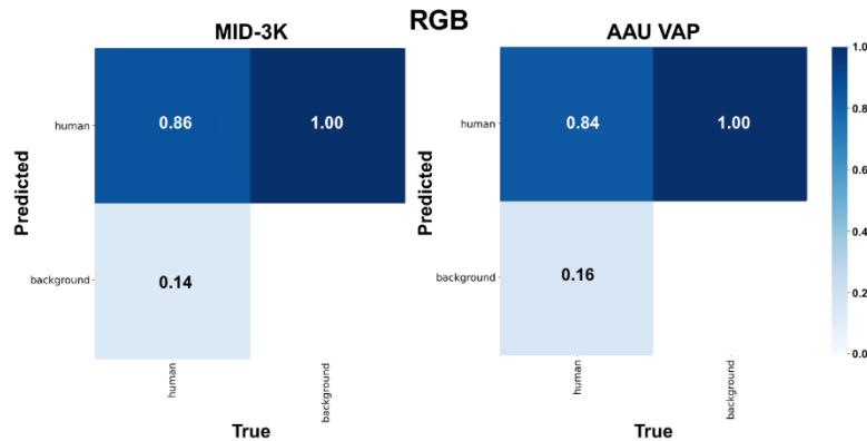
Figure 3.1: Normalized confusion matrices obtained in evaluation of the RGB detector using test splits
