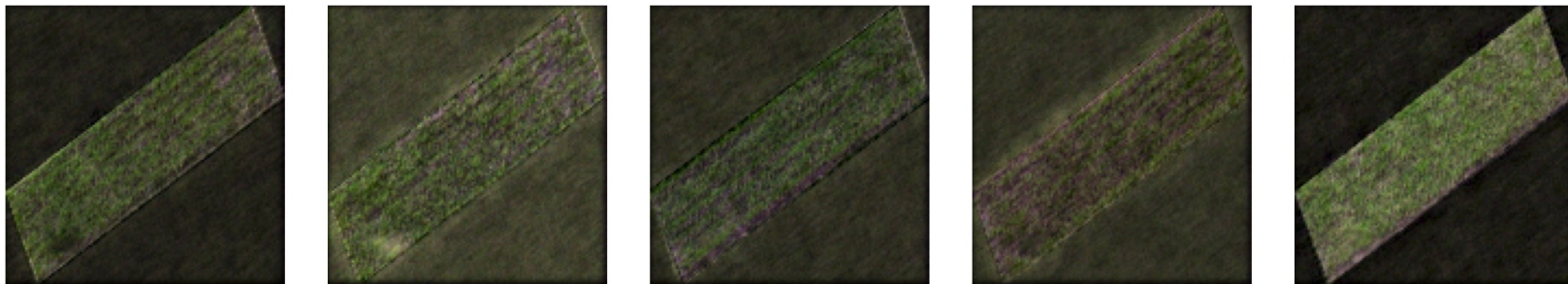
PlantPlotGAN
