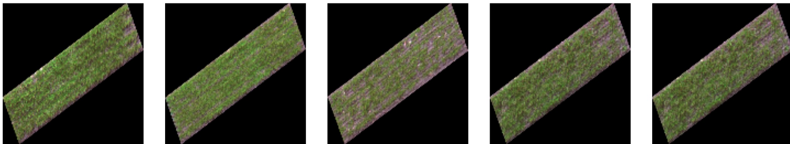
Real images
