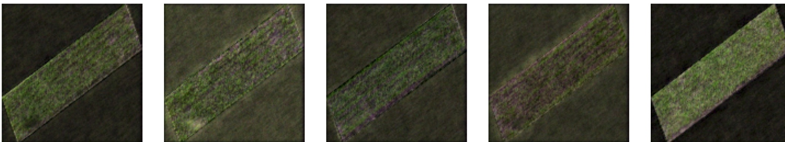
PlantPlotGAN
