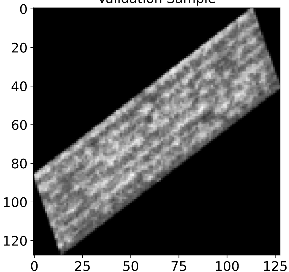
Validation Sample
