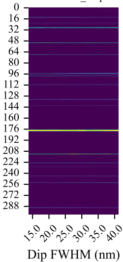
attention_map
