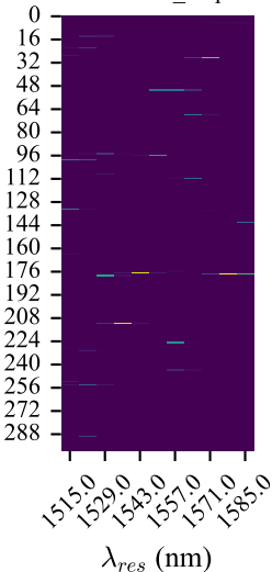
attention_map
