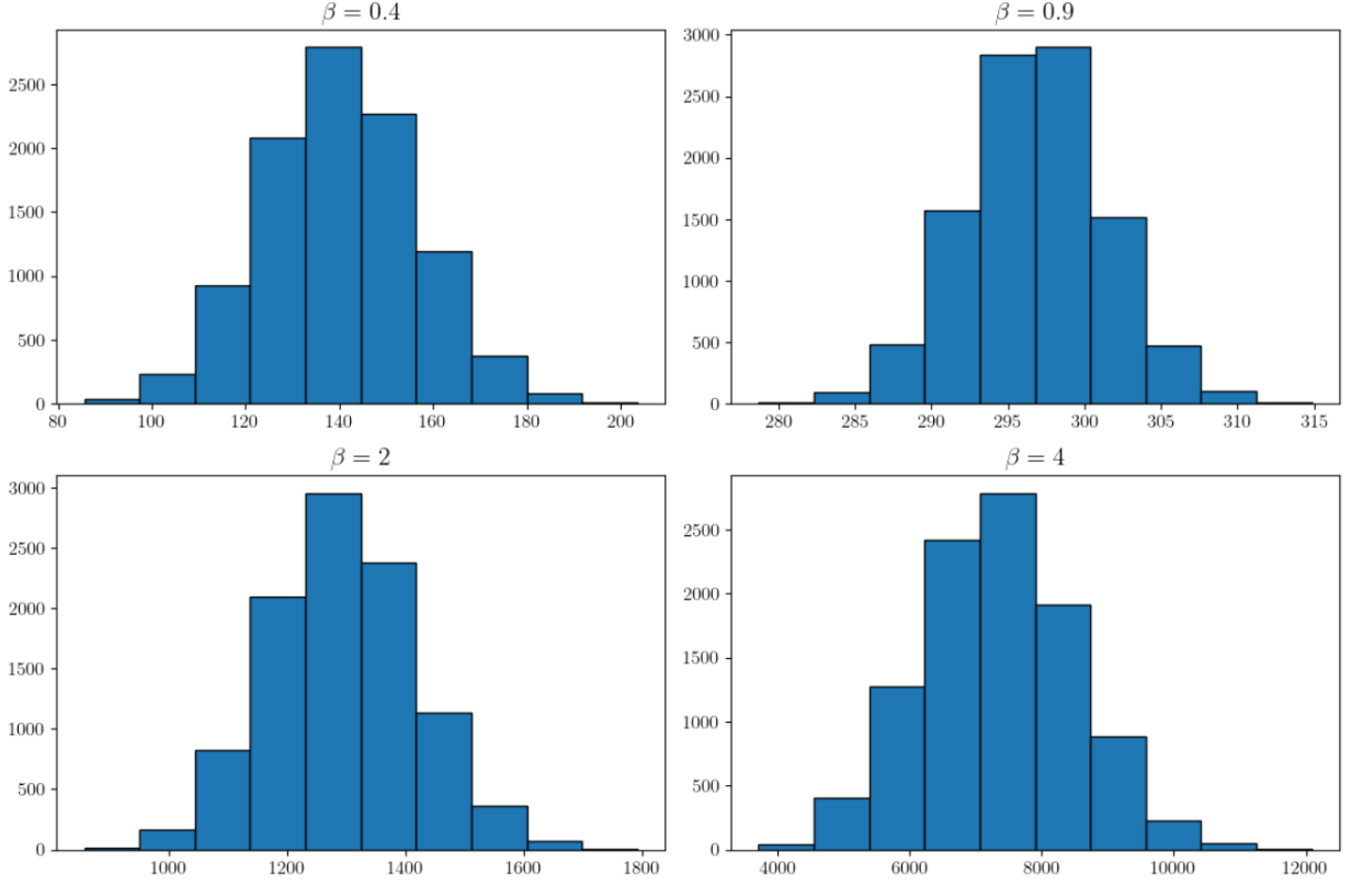
Figure 3: Distribution of F_\beta for p = 64 fixed and \beta \in \{0.4, 0.9, 2, 4\} . To generate the genes, each digit was drawn from the uniform distribution over \{0, 1, 2, 3\} .
