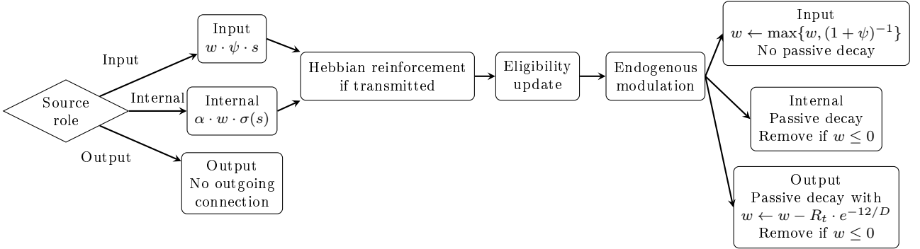
Figure 23: Temporal order of the operations affecting existing connections. Input and internal sources share the plasticity steps but differ in transmission and in the final weight treatment.
