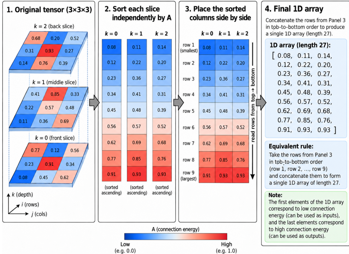
Figure 14: How the ordering works.
