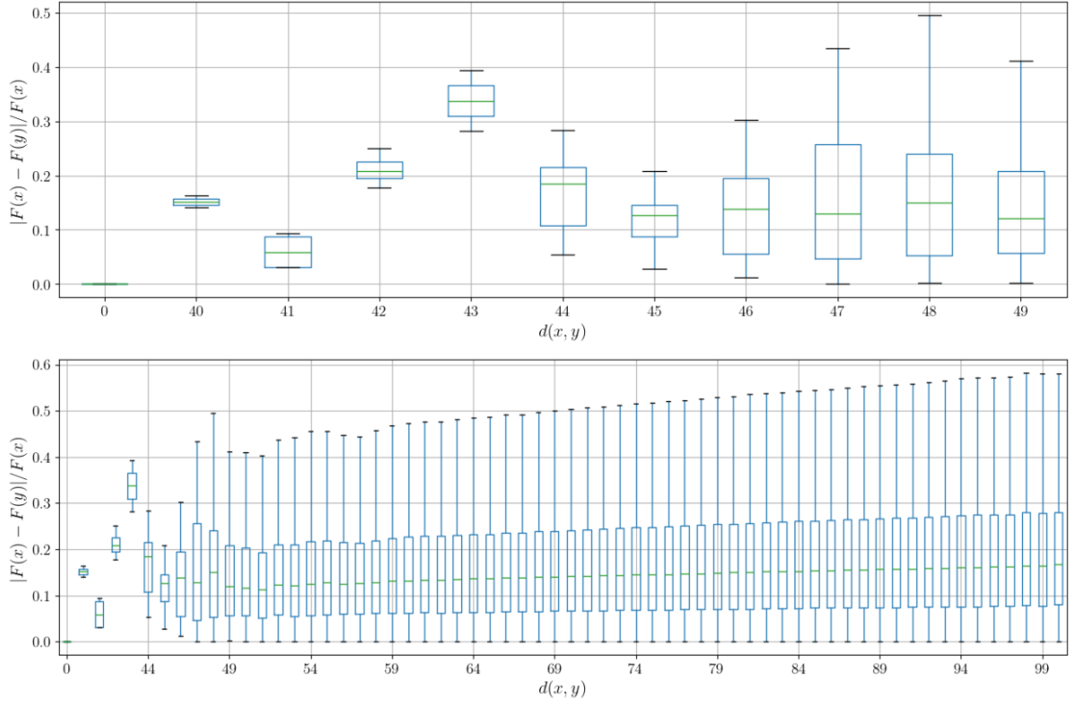
Figure 7: Box plot distribution of the relative differences \frac{|F_\beta(x) - F_\beta(y)|}{F_\beta(x)} for \beta = 4 and 64 digits per gene. The first plot above is a zoomed-in view limited to d(x, y) = 50 for better visualization. The second plot covers the entire range obtained from the samples. To generate the genes, each digit was drawn from the uniform distribution over \{0, 1, 2, 3\} .
