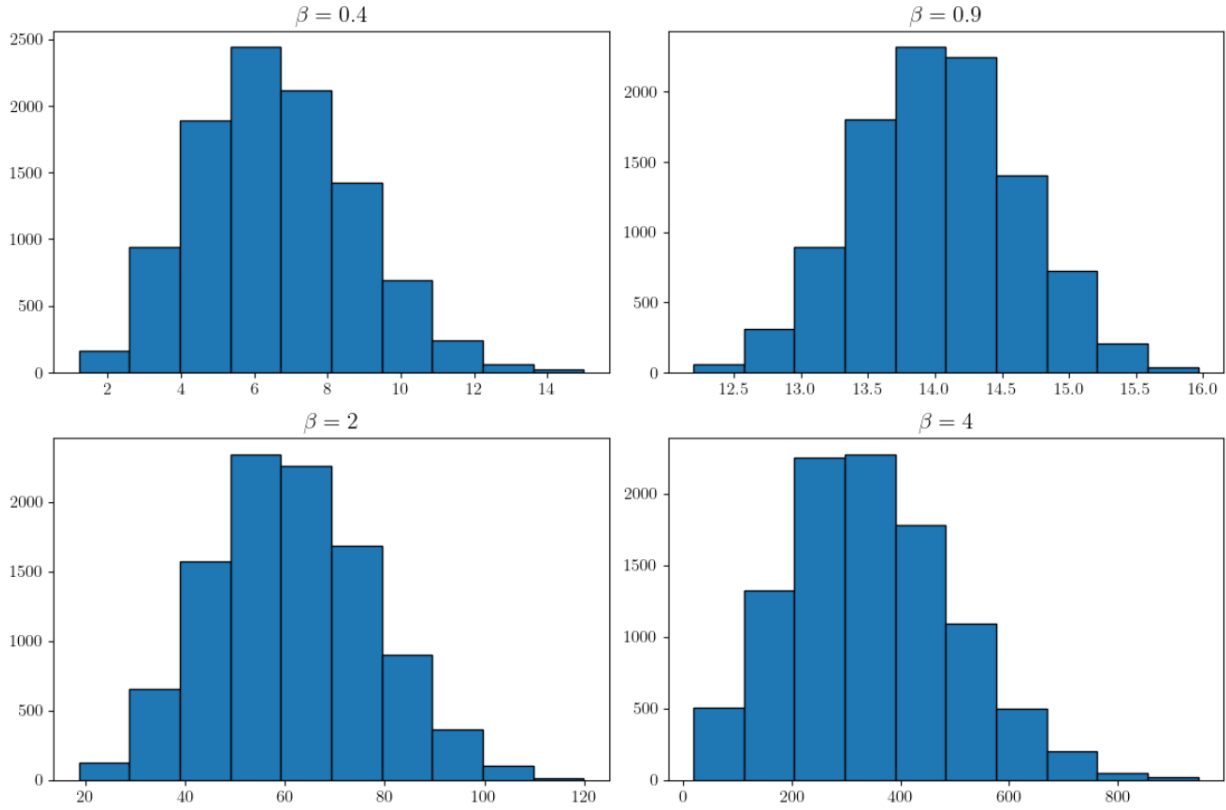
Figure 2: Distribution of F_\beta for p = 8 fixed and \beta \in \{0.4, 0.9, 2, 4\} . To generate the genes, each digit was drawn from the uniform distribution over \{0, 1, 2, 3\} .
