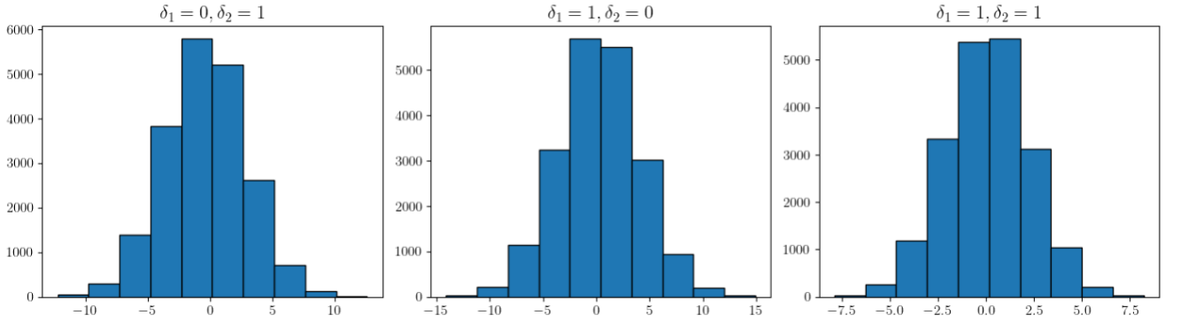
Figure 9: Distribution of G_{\delta_1, \delta_2} for 64 digits per gene. To generate the genes, each digit was drawn from the uniform distribution over \{0, 1, 2, 3\} .
