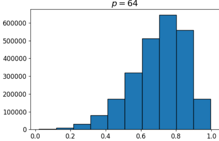
Figure 20: Distribution of M(i, j, k, x) for p = 64, I = 50, J = 50, K = 10 . To generate the genes, each digit was drawn from the uniform distribution over \{0, 1, 2, 3\} .
