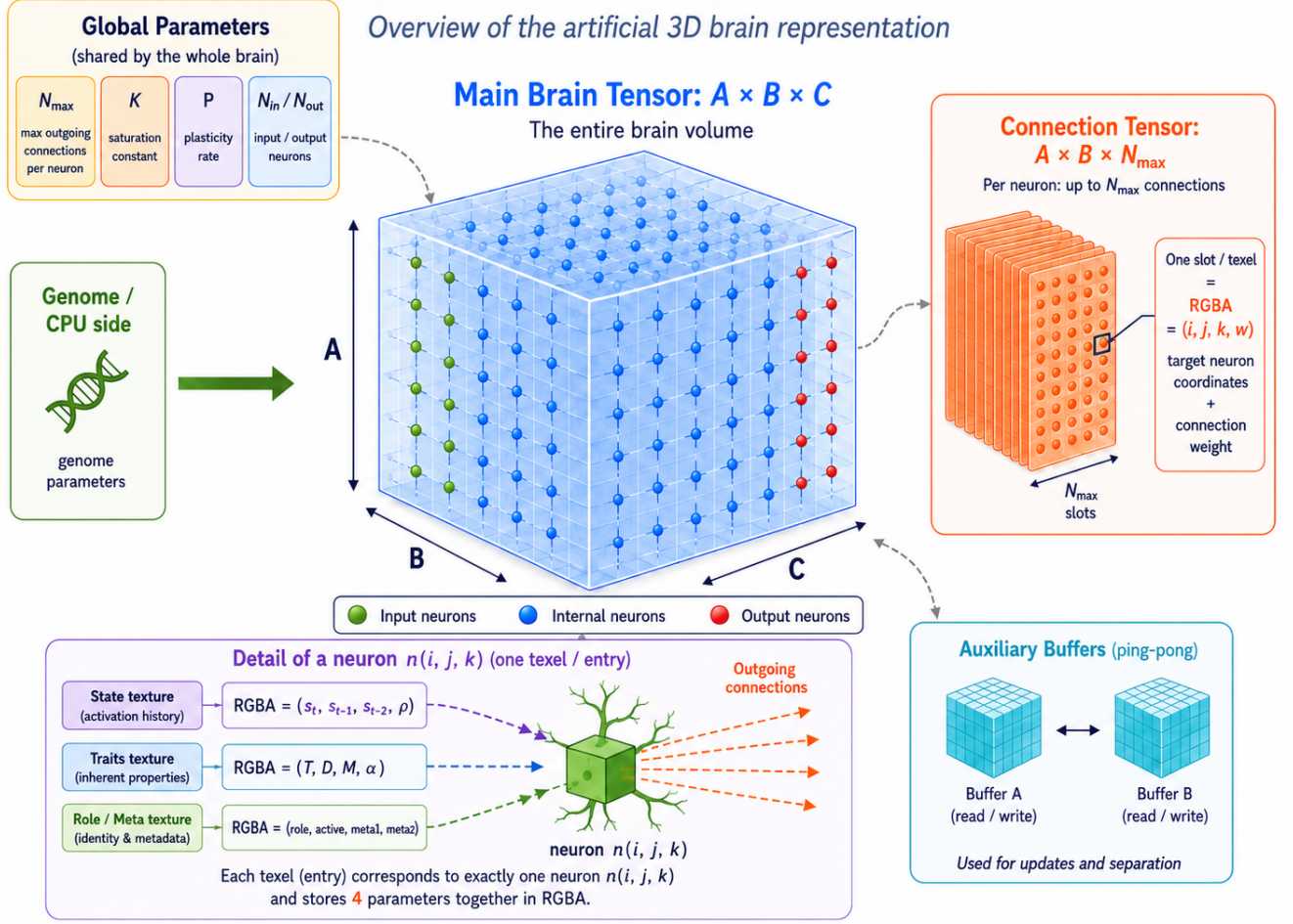
Figure 24: Overview of the brain structure and how its parameters are represented in the GPU.
