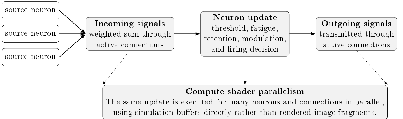
Figure 25: Schematic view of the neuronal dynamics. Each neuron receives weighted signals, updates its internal state, and may then transmit signals through its outgoing connections. Compute shaders are well suited to this model because the same operations can be applied in parallel to large numbers of neurons and connections.
