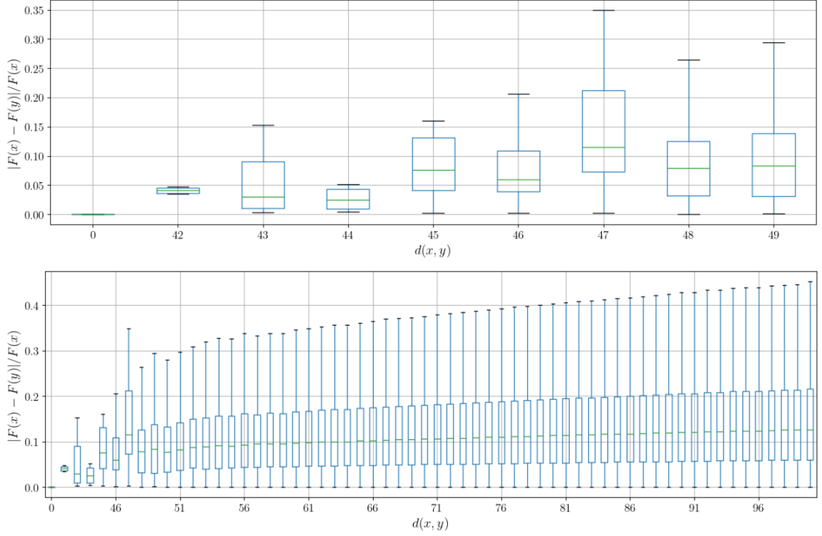
Figure 5: Box plot distribution of the relative differences \frac{|F_\beta(x) - F_\beta(y)|}{F_\beta(x)} for \beta = 0.4 and 64 digits per gene. The first plot above is a zoomed-in view limited to d(x, y) = 50 for better visualization. The second plot covers the entire range obtained from the samples. To generate the genes, each digit was drawn from the uniform distribution over \{0, 1, 2, 3\} .
