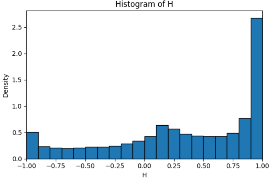
Figure 11: Distribution of H_{i,j,k}(x) for p = 64, I = 50, J = 50, K = 10 . To generate the genes, each digit was drawn from the uniform distribution over \{0, 1, 2, 3\} .
