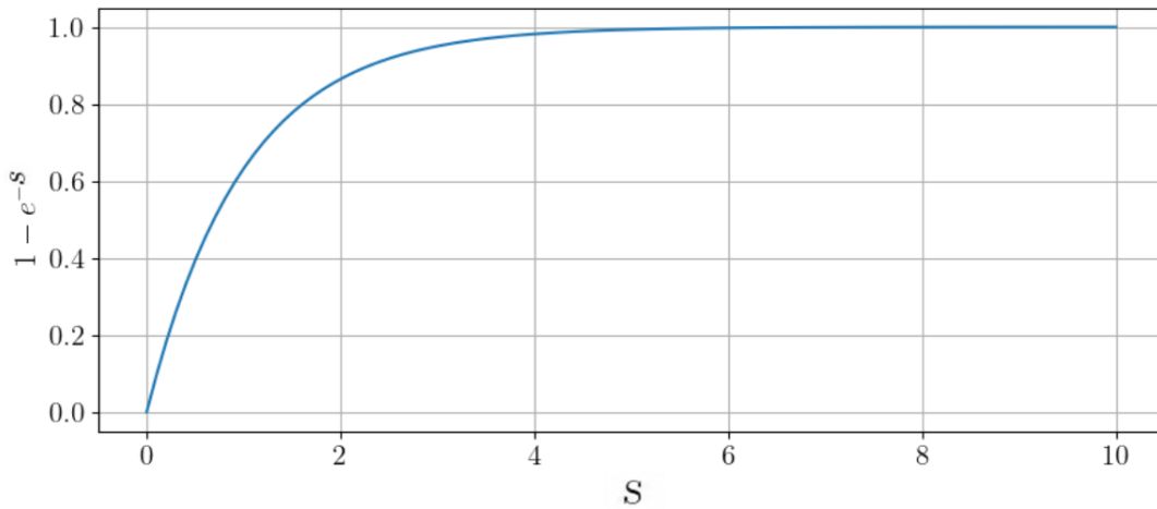
Figure 15: Saturation function \sigma(s) for s \in [0, 10] .
