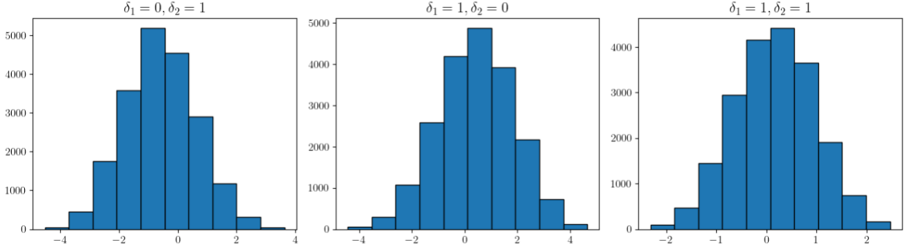
Figure 8: Distribution of G_{\delta_1, \delta_2} for 8 digits per gene. To generate the genes, each digit was drawn from the uniform distribution over \{0, 1, 2, 3\} .
