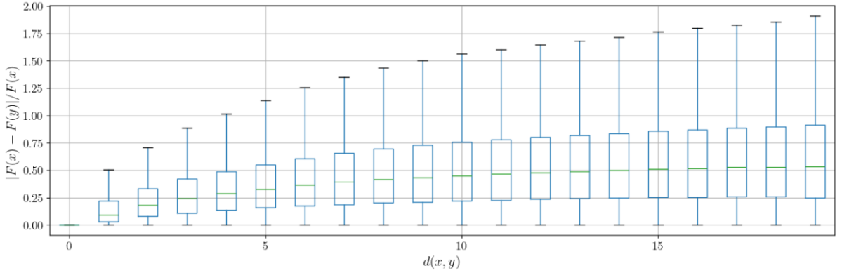
Figure 6: Box plot distribution of the relative differences \frac{|F_\beta(x) - F_\beta(y)|}{F_\beta(x)} for \beta = 4 and 8 digits per gene. To generate the genes, each digit was drawn from the uniform distribution over \{0, 1, 2, 3\} .
