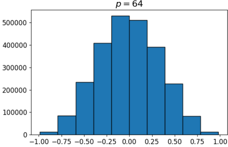
Figure 10: Distribution of A_{i,j,k}(x) for p = 64, I = 50, J = 50, K = 10 . To generate the genes, each digit was drawn from the uniform distribution over \{0, 1, 2, 3\} .
