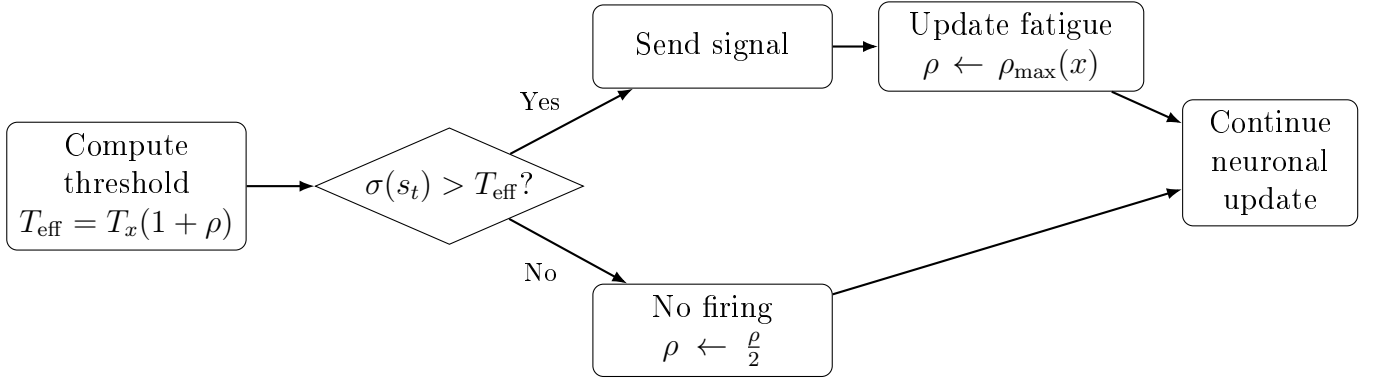
Figure 17: Order of the refractory-state update within one simulation iteration. The current fatigue determines the effective threshold. If the neuron fires, it sends a signal and its fatigue is reset to the genetically determined maximum value \rho_{\text{max}}(x) = F_{0.4}(x) . Otherwise, the fatigue is reduced by half.
