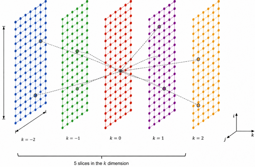
Figure 13: Region of possible connections for a single neuron.
