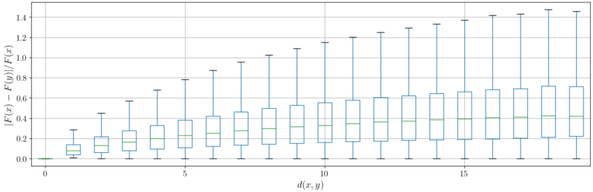
Figure 4: Box plot distribution of the relative differences \frac{|F_\beta(x) - F_\beta(y)|}{F_\beta(x)} for \beta = 0.4 and 8 digits per gene. To generate the genes, each digit was drawn from the uniform distribution over \{0, 1, 2, 3\} .
