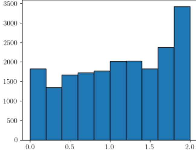
Figure 22: Distribution of the input influence factors 1 + \sin(G_{1,1}(x)) . To generate the genes, each digit was drawn from the uniform distribution over \{0, 1, 2, 3\} .
