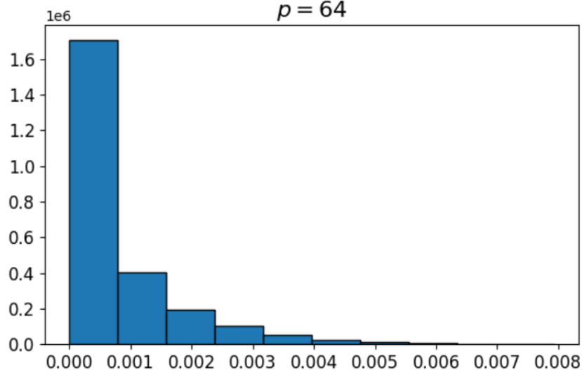
Figure 19: Distribution of e^{-12/D(i,j,k,x)} for p = 64, I = 50, J = 50, K = 10 . To generate the genes, each digit was drawn from the uniform distribution over \{0, 1, 2, 3\} .
