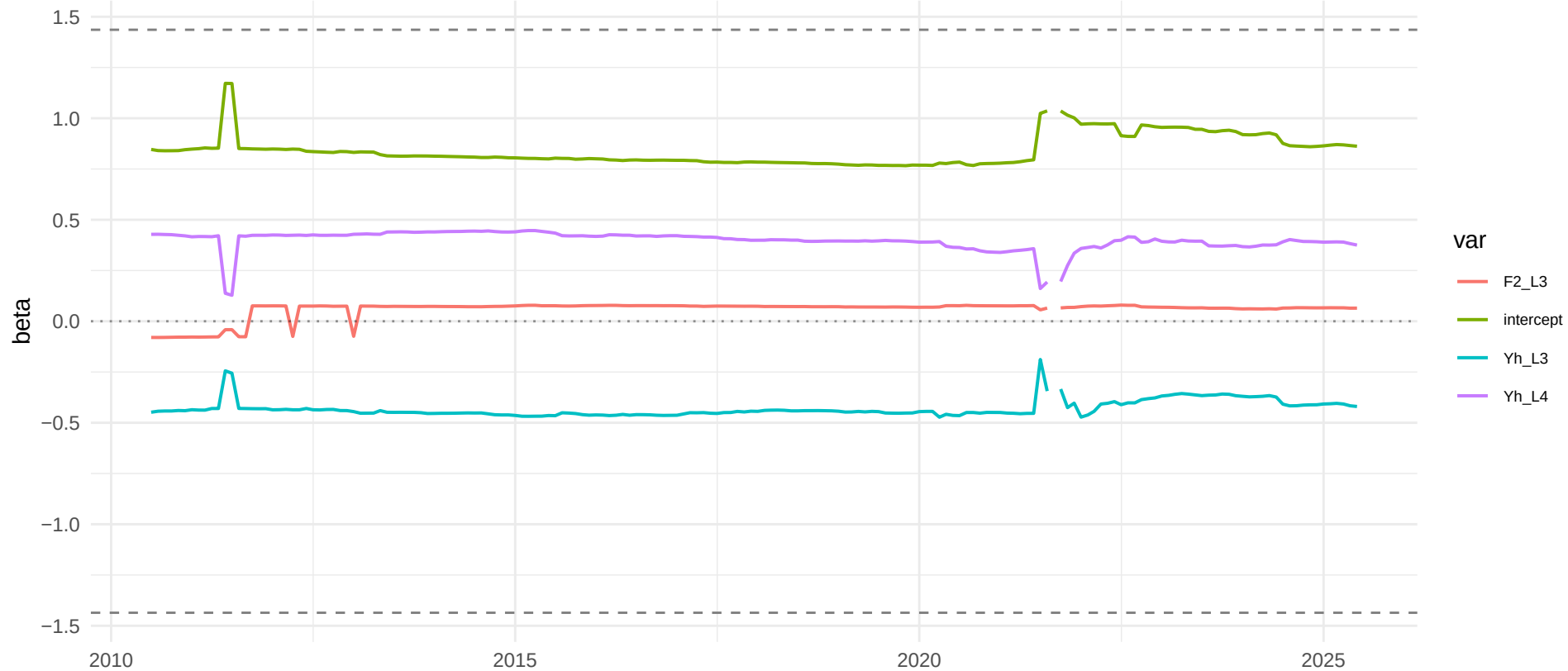
h=3: top-4 TVP (FAVAR) betas vs constant Ridge ( |\text{beta}|=1.436 )
