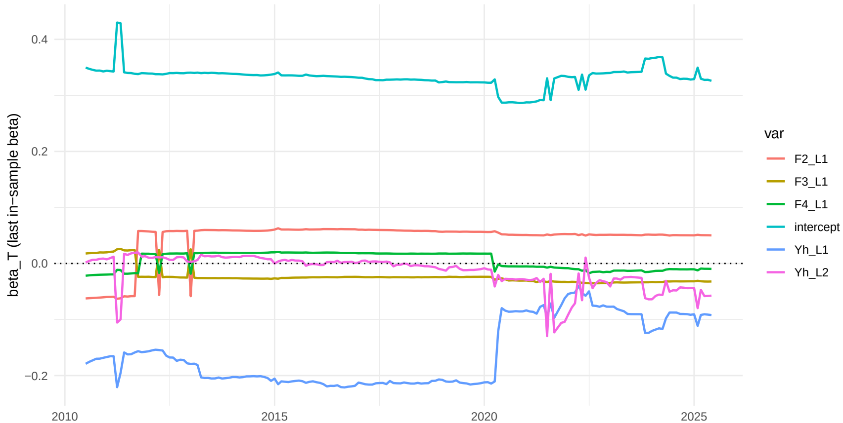
TVP-FAVAR, h=1: top-6 betas (by sd)
