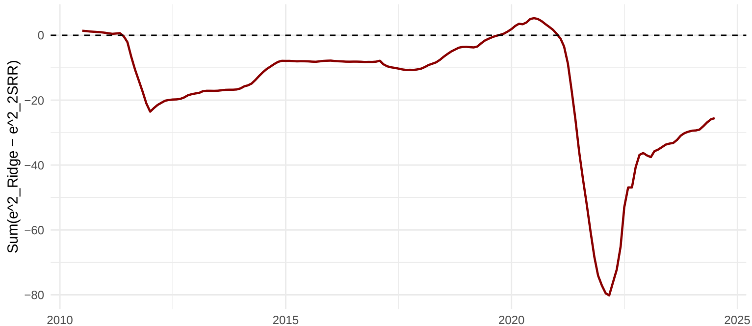
CSSED 2SRR-AR vs Ridge Step1, h=12
