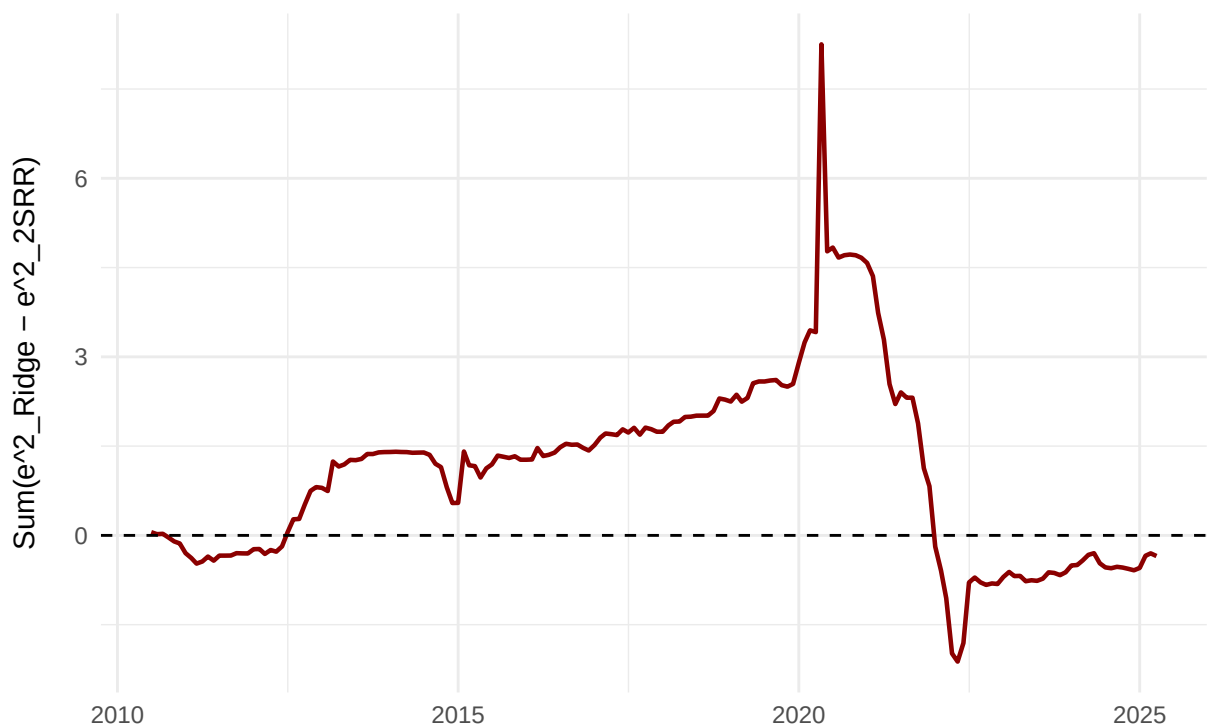
CSSSED 2SRR-FAVAR vs Ridge Step1, h=3
