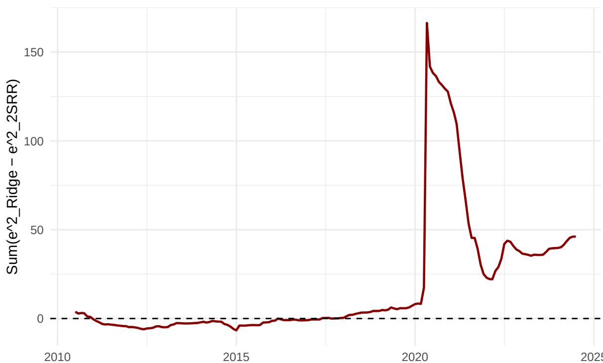
CSSSED 2SRR-FAVAR vs Ridge Step1, h=12
