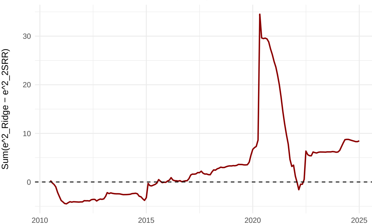
CSSSED 2SRR-FAVAR vs Ridge Step1, h=6
