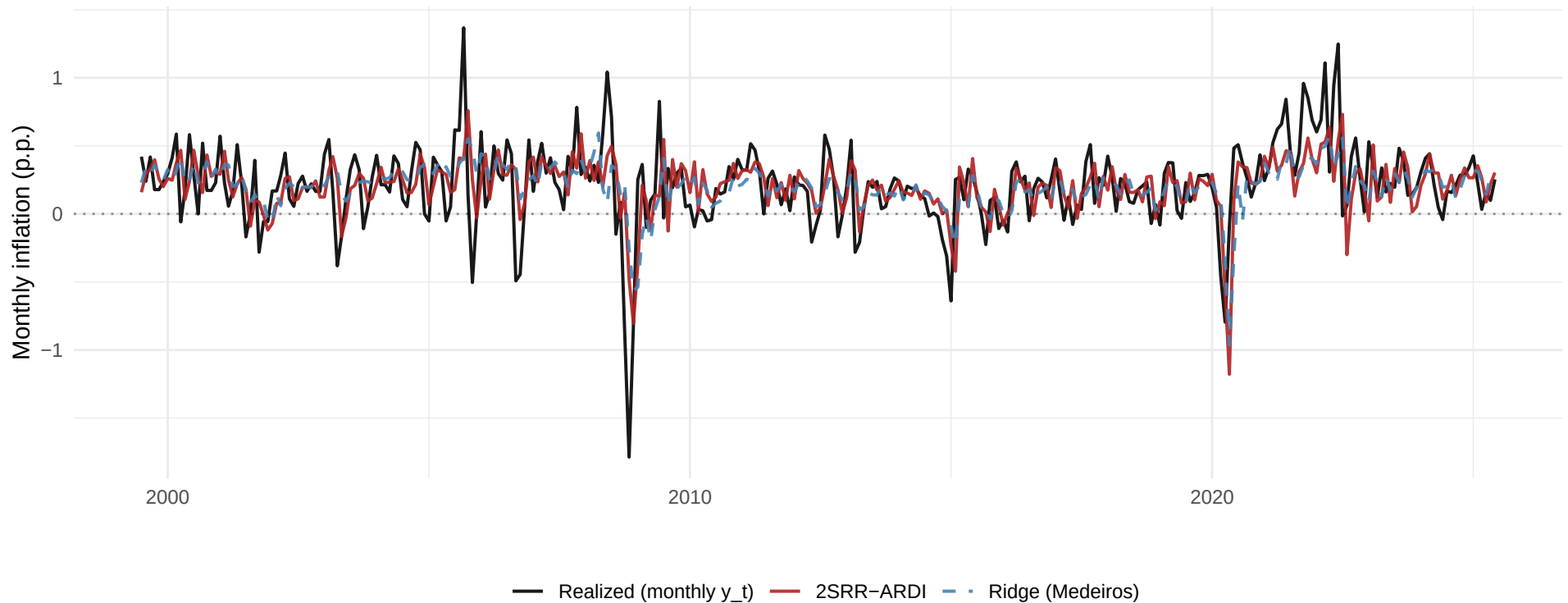
2SRR-ARDI vs classical Ridge (Medeiros), h=1
