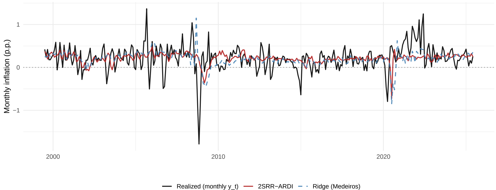
2SRR-ARDI vs classical Ridge (Medeiros), h=3
