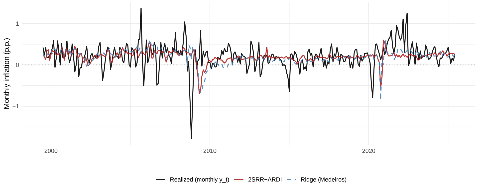
2SRR-ARDI vs classical Ridge (Medeiros), h=6
