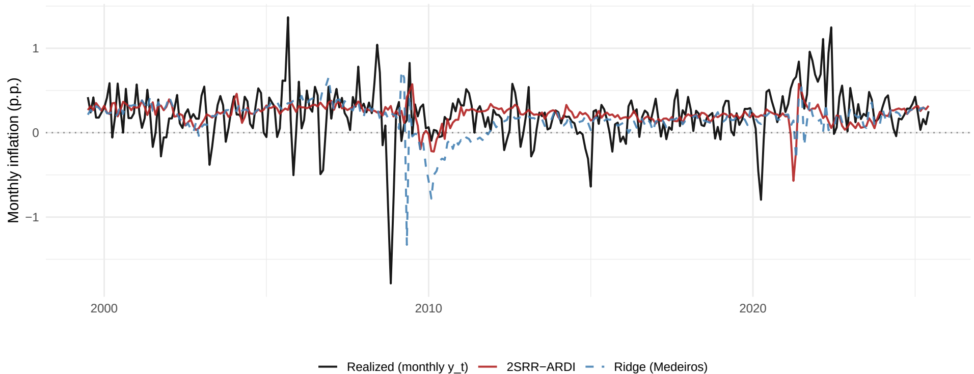
2SRR-ARDI vs classical Ridge (Medeiros), h=12
