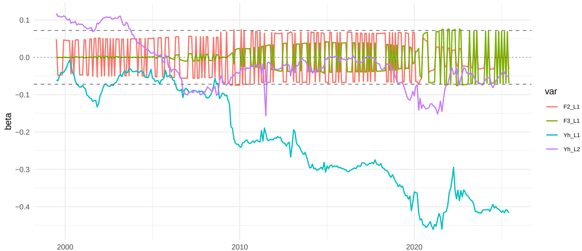
h=1: top-4 TVP (ARDI) betas vs constant Ridge ( |\text{beta}|=0.072 )
