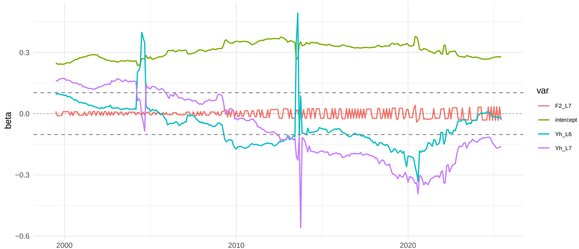
h=6: top-4 TVP (ARDI) betas vs constant Ridge ( |\text{beta}|=0.102 )
