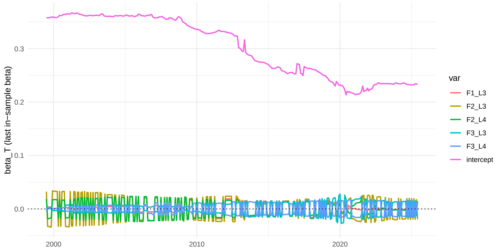
TVP-Factor, h=3: top-6 betas (by sd)
