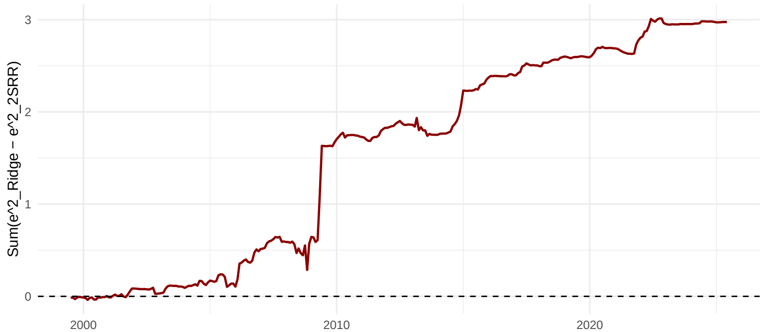
CSSED 2SRR-AR vs Ridge Step1, h=6
