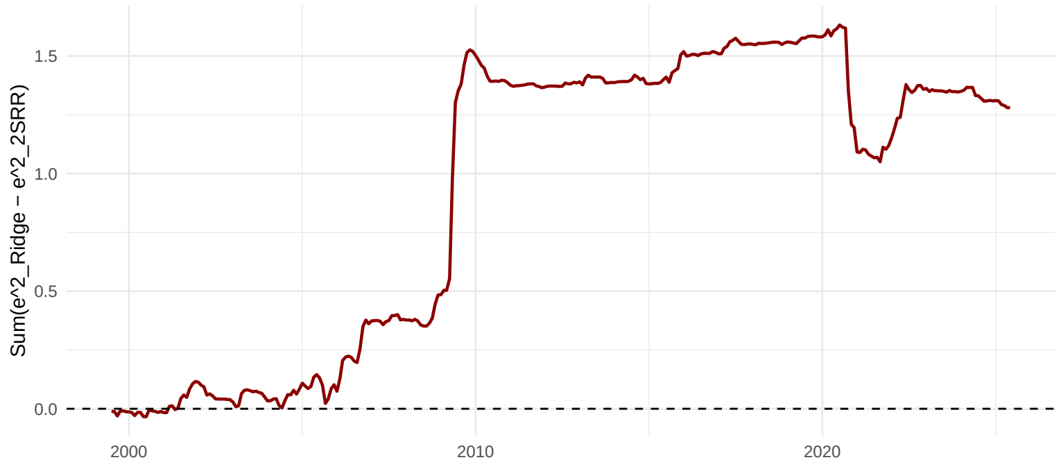
CSSED 2SRR-Factor vs Ridge Step1, h=6
