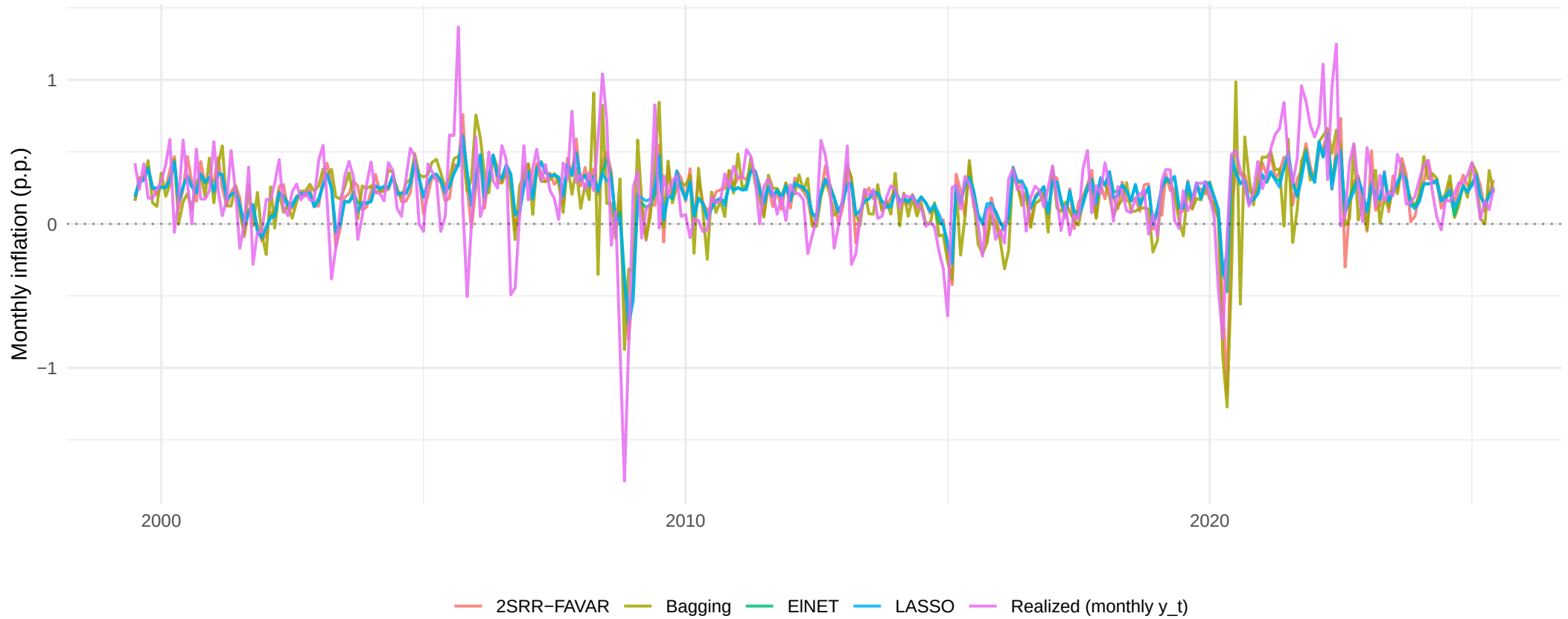
Forecasts h=1 (monthly scale): 2SRR-FAVAR + 2 best + worst Medeiros
