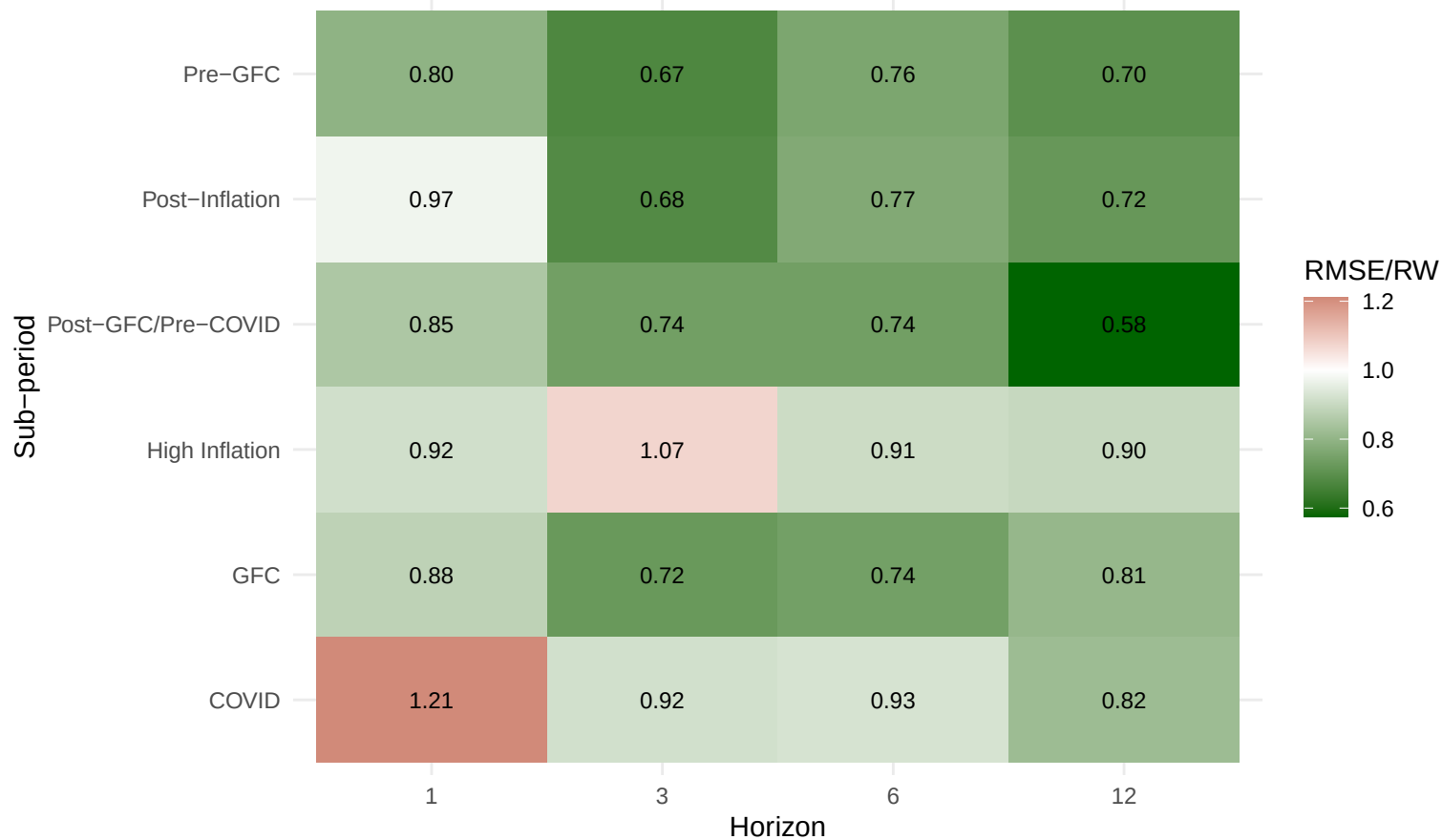
TVP-ARDI: RMSE relative to RW per sub-period
