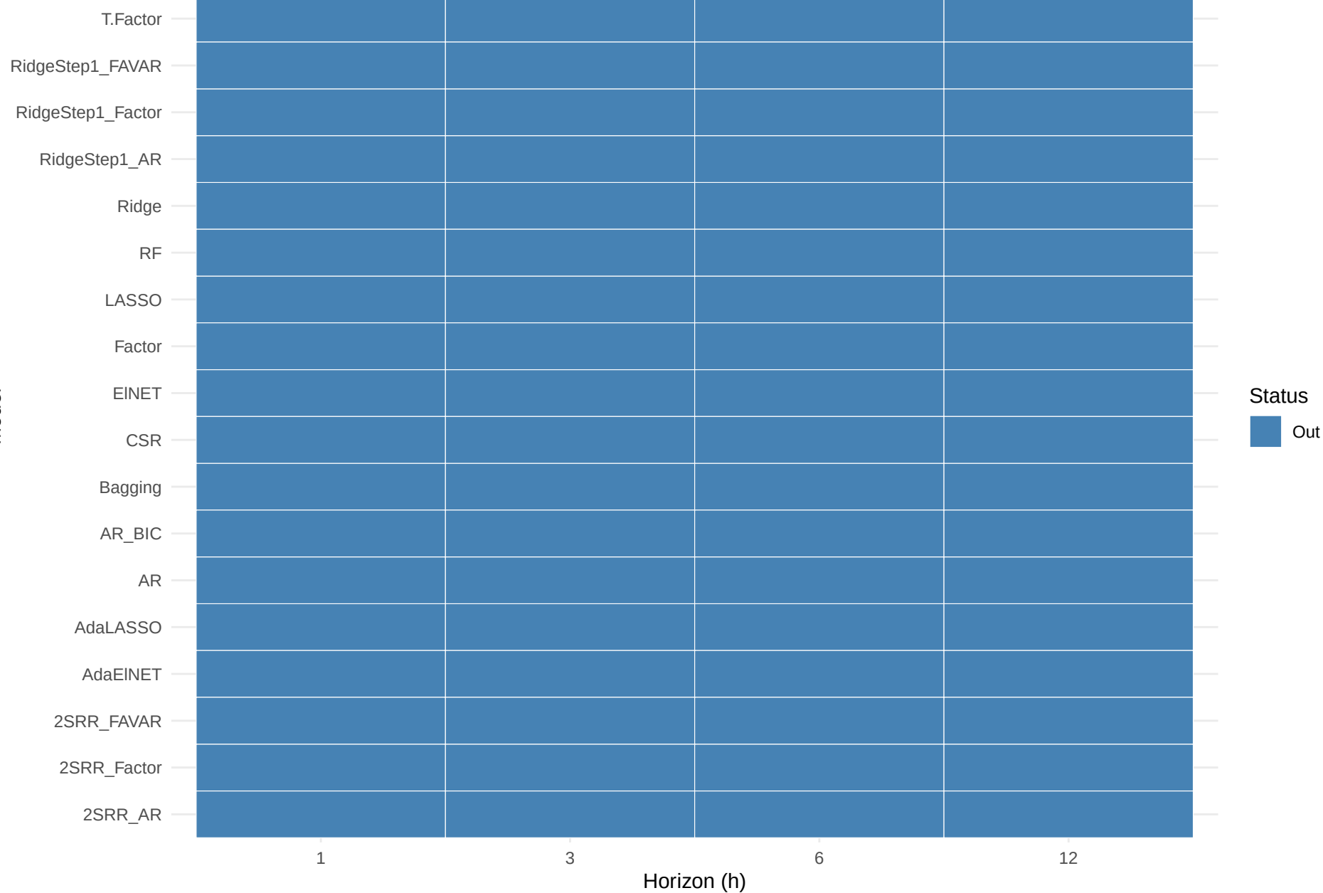
Model Confidence Set per horizon
