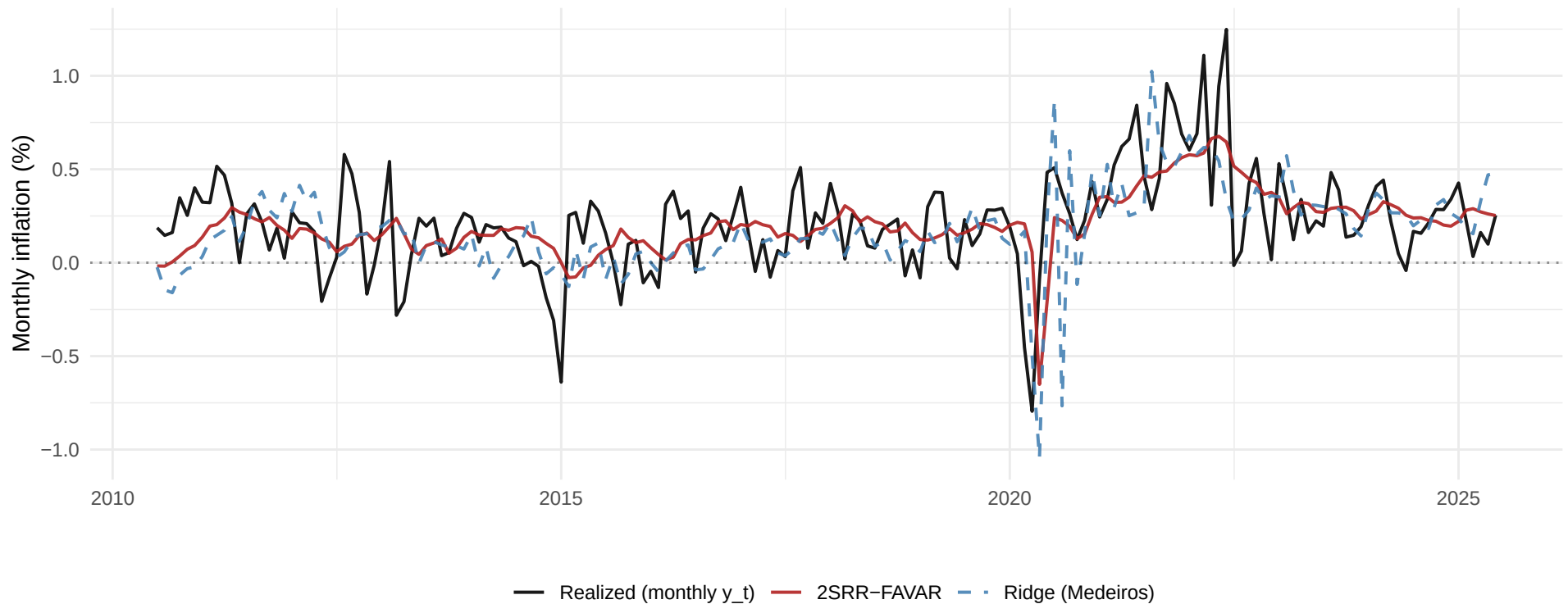
2SRR-FAVAR vs classical Ridge (Medeiros), h=6
