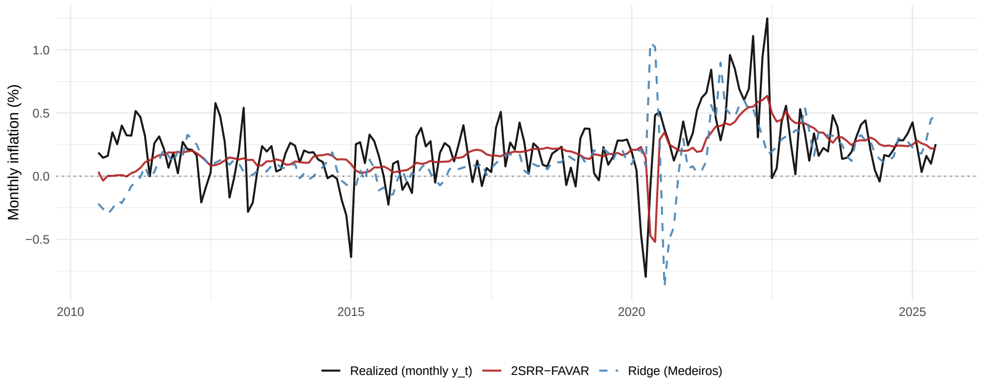
2SRR-FAVAR vs classical Ridge (Medeiros), h=12
