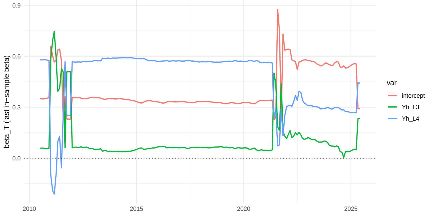
TVP-AR, h=3: top-3 betas (by sd)
