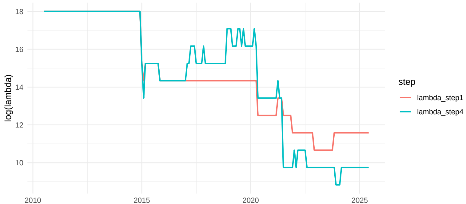
TVP-FAVAR, h=1: Step1 vs Step4 lambdas (log)
