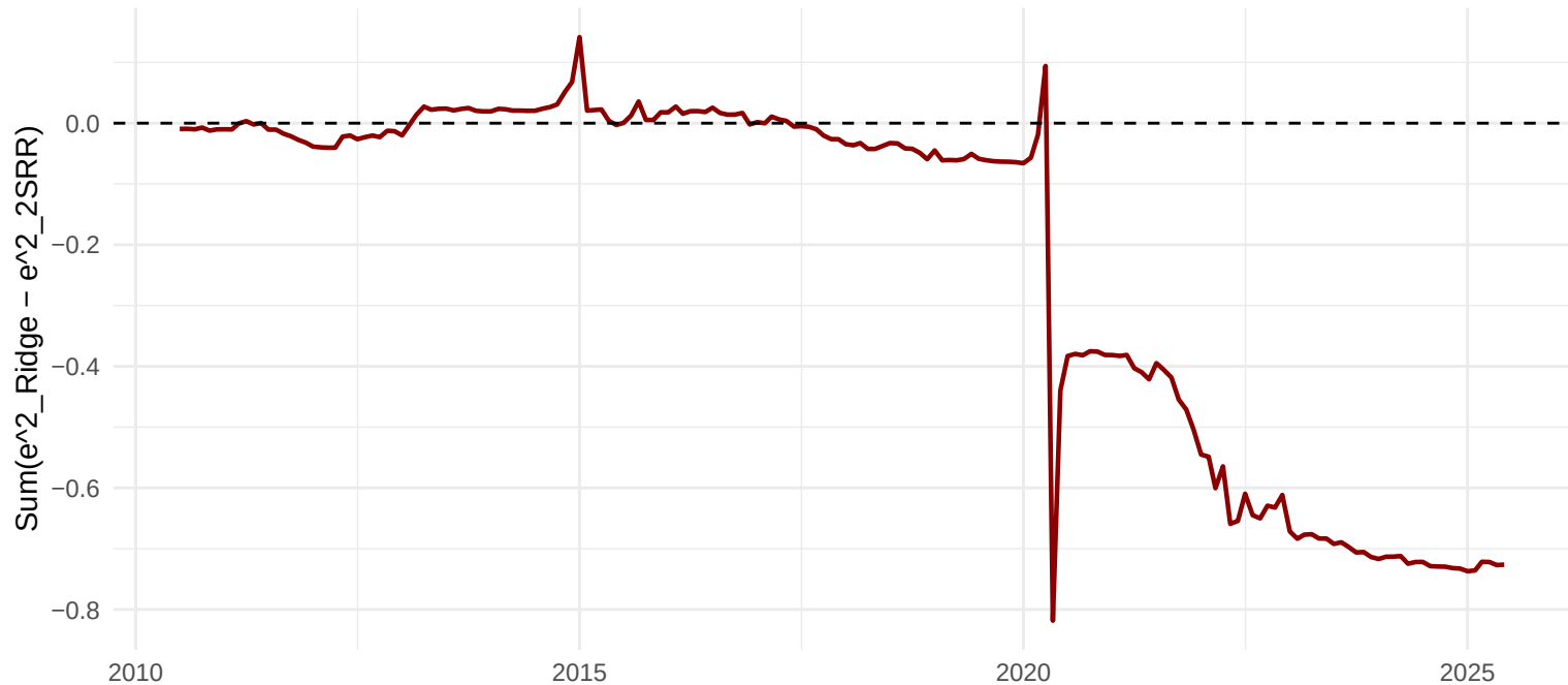
CSSSED 2SRR-FAVAR vs Ridge Step1, h=1
