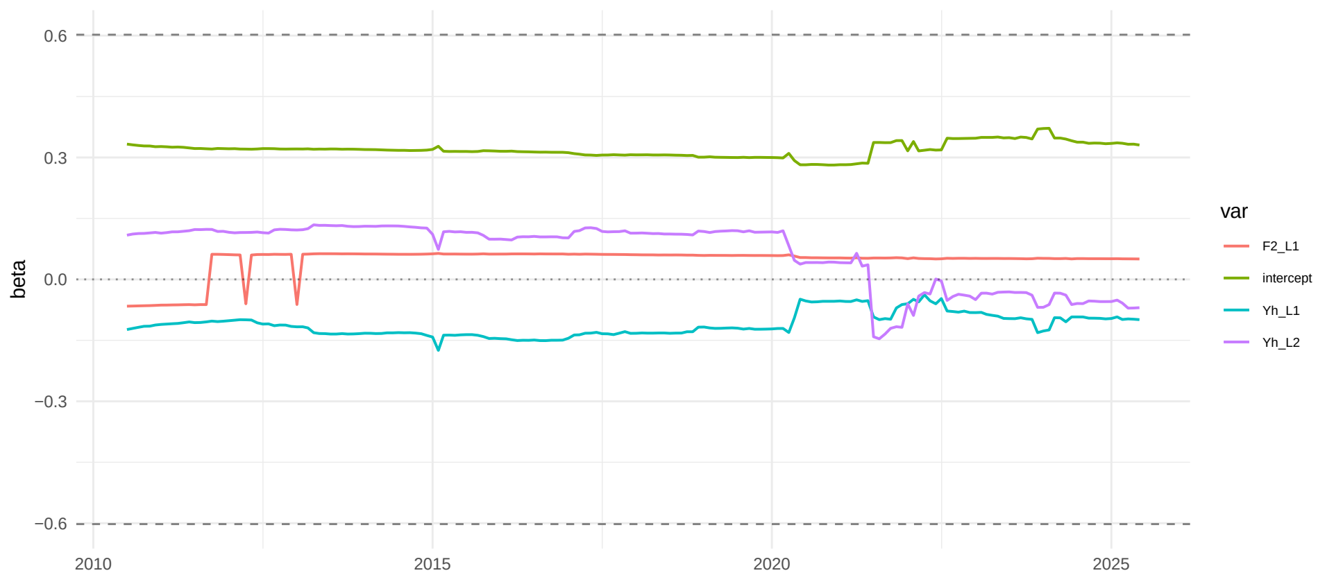
h=1: top-4 TVP (FAVAR) betas vs constant Ridge ( |\beta|=0.602 )
