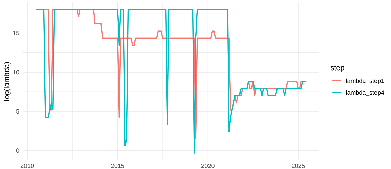
TVP-AR, h=1: Step1 vs Step4 lambdas (log)
